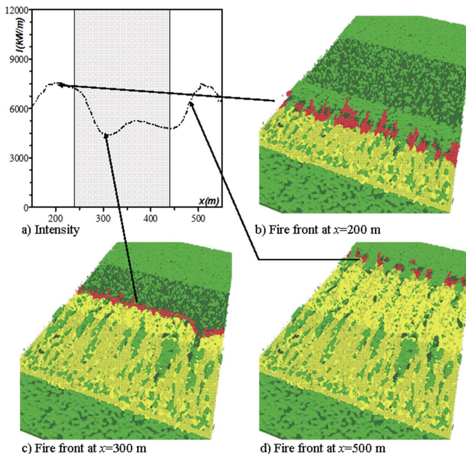
Figure 10. Numerical simulation of a fire spreading over a fuel break in a Pinus halepensis stand, using the coupled fire-atmosphere model FIRETEC (INRA – LANL joint work, Pimont et al. 2008). Cover fraction of trees on the fuel break is 25%. The fire spreads along the x -axis and the fuel-break extends from x=240 m to x=440 m. Flame contours in red are deduced from computed isotherms. Green and yellow colour contours are used respectively for tree canopy and surface fuels (shrubs, grasses) representations (iso-contours of computed biomass density).
