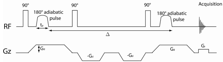
Fig. 6: One-dimensional DOSY pulse sequence [44]. Two negative gradient pulses are added to reduce eddy currents. t_p is the adiabatic pulse duration, G_d and G_r are, respectively, the intensity of the diffusion and read gradients, and \Delta is the diffusion time.
