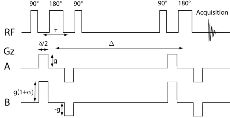
Fig. 1: PGSE pulse sequences that use composite pulses. A , classical BPPLIED sequence B , the pulse sequence designed by Morris et al. [16] that uses unequal gradient pulses in each bipolar pair. Additional gradient pulses can be used in B to refocus the lock signal and to dephase unwanted coherences. Spoil gradients can also be added to the BPPLIED pulse sequence. RF denotes the radio-frequency time train and Gz the gradient pulse time train. \delta is the gradient duration, g is the gradient amplitude, \Delta is the diffusion time (midpoints of the two diffusion encoding periods), \tau is the time between the midpoints of the antiphase field gradients, and \alpha is the unbalancing factor of the gradient pulses.
