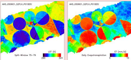
Figure 1: Land Surface Temperature (LST) and daily Evapo-Transpiration (ET) retrieved from Airborne Hyperpectral Scanner (AHS) data over the Barrax agricultural area in the framework of the Sen2flex-2005 campaign.
