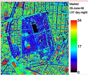
Figure 2: Difference between LST at night over the Madrid city (DESIREX-2008) retrieved from AHS data
