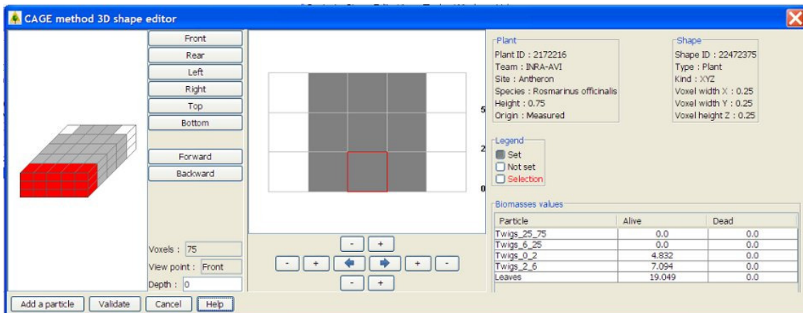
Figure 84: Measured 3D shape edition without voxel types
