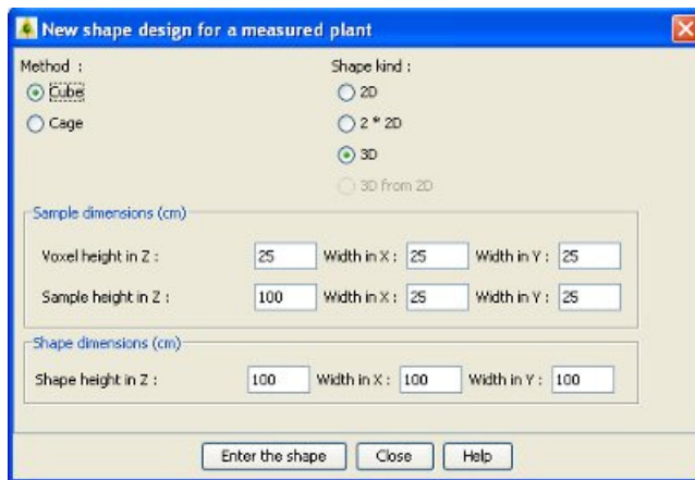
Figure 78: Measured plant shape creation
