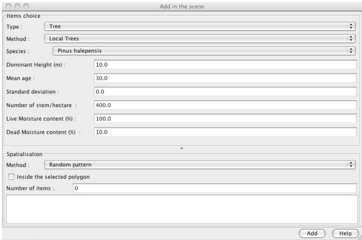
Figure 20: Adding a Local Tree
