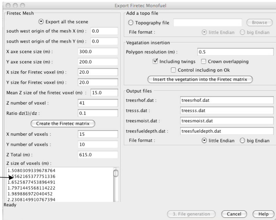
Figure 55: FIRETEC Export Interface. The left column is dedicated to FIRETEC mesh computation. The right column contains the options available for export (inclusion of a topography, Resolution of the 3D Matrix of Fuel LayerSets, etc.) and file names.
