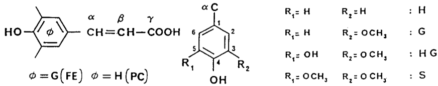
Fig. 1. Molecular structure of the most frequent cell wall-linked phenyl propenoic acids ( \phi = H or G ). Corresponding phenylpropenoid alcohols provide the monomeric units of the lignin macromolecular network.
