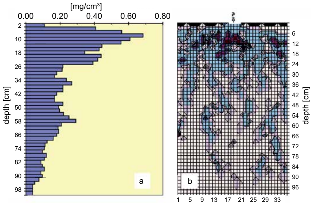
Fig. 1. Root profile distribution expressed as a) dry mass density and b) index related to the number and size of the visible roots per square ( Zea mays L., Sarnevo, Bulgaria, 1993).
