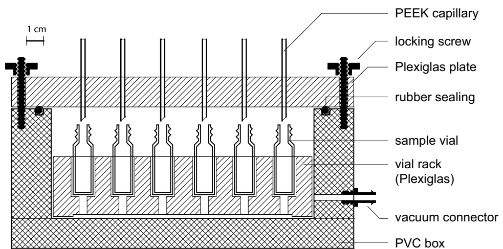
Fig. 2: Vacuum device for collecting samples (from Göttelein et al. 1996; with permission from Elsevier)
