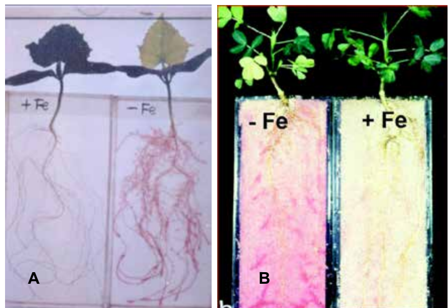
Fig. 1: FeII reduction along roots of cucumber (A) grown in hydroponics and of peanut in rhizobox culture (B) with or without Fe supply. Detection by formation of red Fe^{2+} complexes with BPDS.
