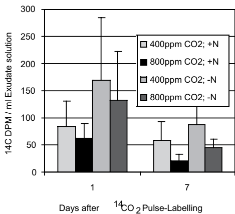
Fig. 2: Localized collection of 14 C-labeled root exudates collected with paper discs (∅ 5 mm, see Fig.1) in 1 cm apical root zones after 14 CO 2 shoot pulse-labelling of bean plants grown in rhizobox culture depending on N supply and atmospheric CO 2 concentration.
