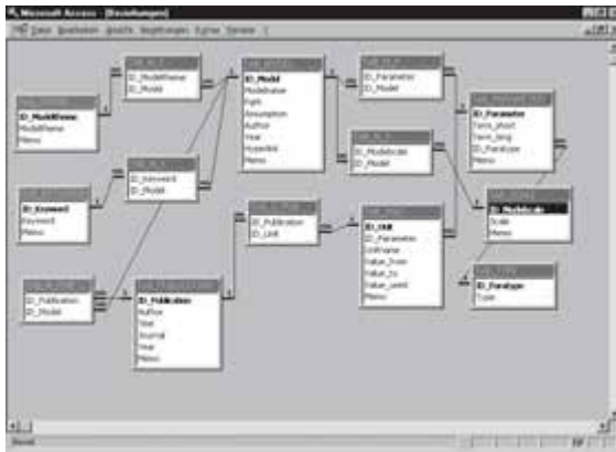
Fig. 1. Entity-Relationship Diagram
