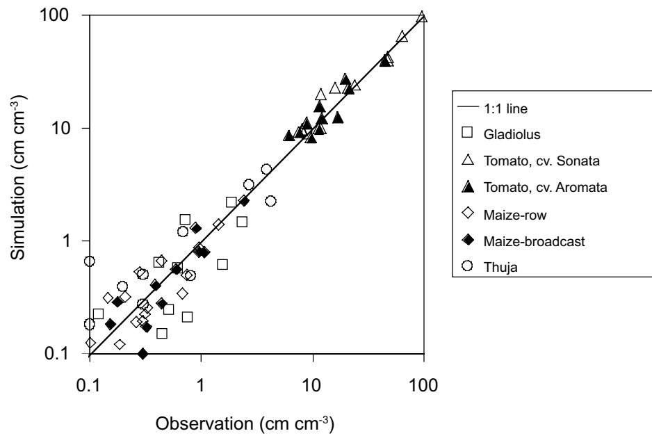
Fig. 1: Observed and simulated root length densities for different crops (from Heinen et al., 2003; with kind permission of Springer Science and Business Media).
