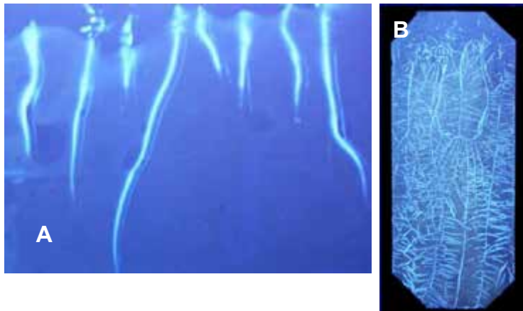
Fig.1: Fluorescent phenolics released along the main root of cowpea seedlings germinated in filter paper (A) and from roots of soil-cultured Phaseolus vulgaris in rhizoboxes (B). Collection by 20-application of a nylon membrane onto the root surface.
