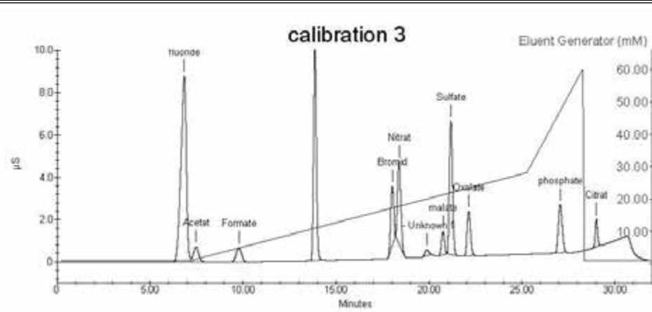
Fig.1: Chromatogram of a calibration of 11 anions and low-molecular-weight acids measured by IC
