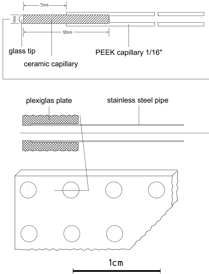
Fig. 1: Details of micro suction cups and their installation (from Göttelein et al. 1996; with permission from Elsevier)
