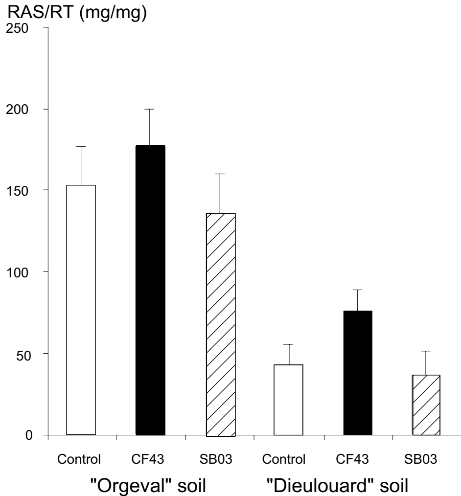
Fig. 1. Effect of wheat inoculation with P. polymyxa strains. CF43 is wild type levan producer (EPS +) and SB03 its mutant whose sacB gene encoding levansucrase is disrupted (EPS -). Levan is a fructosyl polymer. Pot experiment was carried out with two french cultivated soils: Orgeval soil, 6% sand, 76% silt, 15% clay, pH 6.6 and Dieulouard soil, 36% sand, 48% silt, 12% clay, pH 5.6. Before utilisation, soil samples were air-dried, sieved to 4 mm, and sterilized by gamma radiation. RAS/RT ratios are represented by bars derived from the means of n = 14 to 24 replicates depending on treatments. Error bars show confidence intervals (P = 0.05). (from Bezzate et al. 2000; with permission of Blackwell Publishing)
