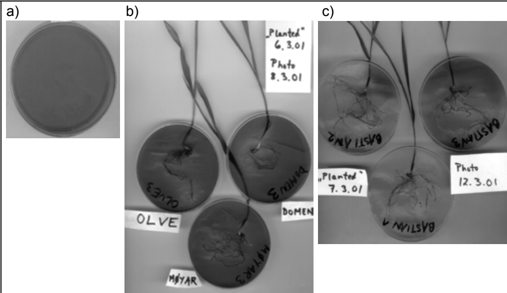
Fig. 1: At pH 7, the agar is greyish-pink (a). In total, 35 varieties of barley and 17 of wheat were compared. The N-source was nitrate, and hence a pH increase was to be expected. In general, pH increased in barley (blue agar; b), but decreased in wheat (yellow agar, c).
