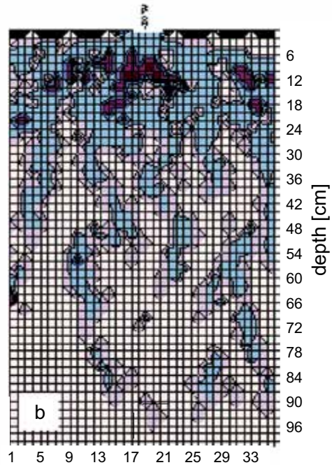
Fig. 1. Root profile distribution expressed as a) dry mass density and b) index related to the number and size of the visible roots per square ( Zea mays L., Sarnevo, Bulgaria, 1993).
