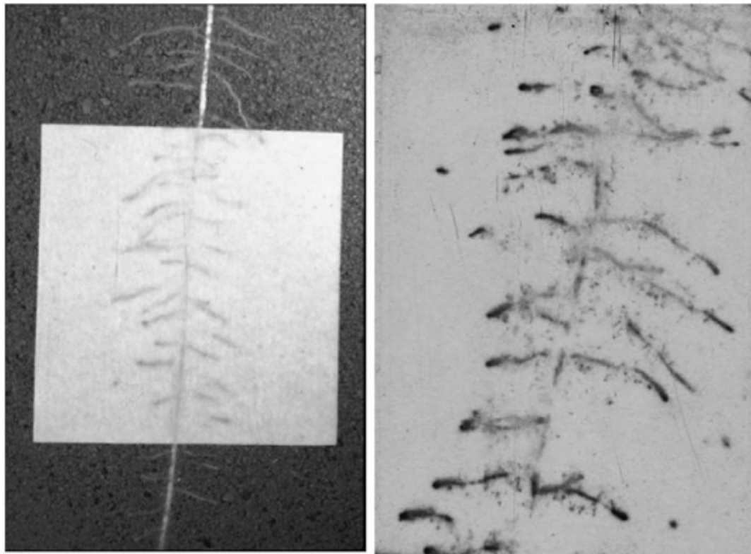
Acid phosphatase activity in the rhizosphere of soil-grown plants in rhizobox-culture by application of filter paper soaked with naphthyl-phosphate. Fast-Red TR substrate solution.
