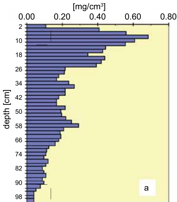
Fig. 1. Root profile distribution expressed as a) dry mass density and b) index related to the number and size of the visible roots per square ( Zea mays L., Sarnevo, Bulgaria, 1993).
