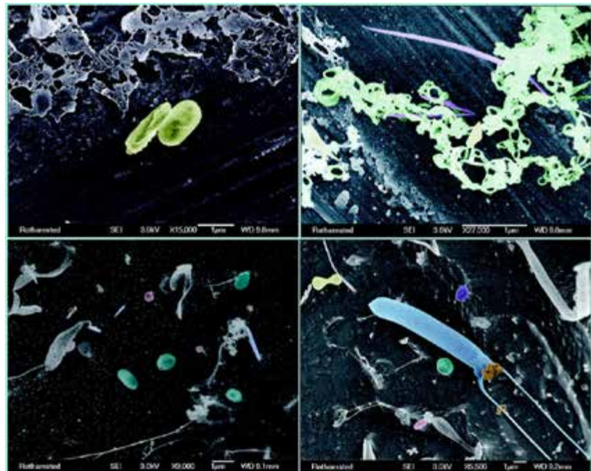
Fig. 3 False colour scanning electron micrographs of cryo-fixed, chromium coated microsample contents. Images demonstrate diverse range of sizes and morphologies of microorganisms. We thank Jean Devonshire (Rothamsted Research) for assistance.
