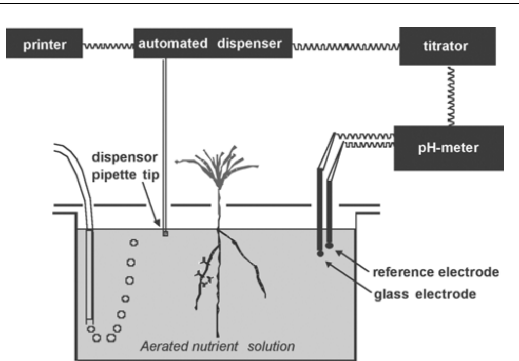
Fig. 1. Experimental set-up for continuous monitoring of proton efflux/influx from roots grown in hydroponics at a given pH values (pH-stat device).
