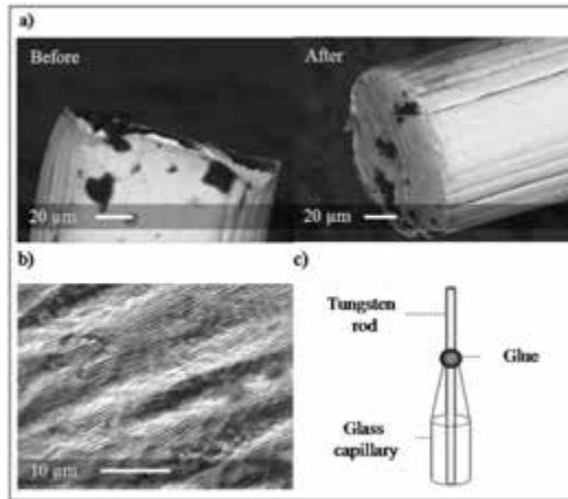
Fig. 1 Scanning electron micrographs of: (a) tungsten rod before and after laser cutting; (b) cut end of tungsten rod; (c) diagram of micro-sampler assembly.
