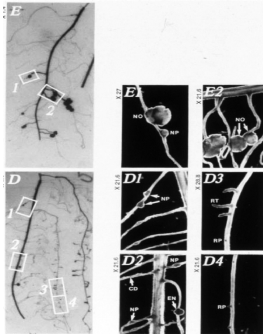
Figure 1. Autoradiographs and corresponding details on stained roots of the E-early and D- delayed inoculated split-root system of soybean. Abbreviations: NO – nodules, EN- emerging nodule, NP- nodule primordia, CD-cortical cell division centres, RP-root primordia, RT-root tips (from Hacin et al., 1997; reproduced with permission of the New Phytologist Trust).
