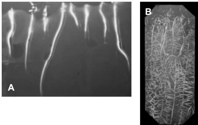
Fig. 1: Fluorescent phenolics released along the main root of cowpea seedlings germinated in filter paper (A) and from roots of soil-cultured Phaseolus vulgaris in rhizoboxes (B). Collection by 20-application of a nylon membrane onto the root surface.
