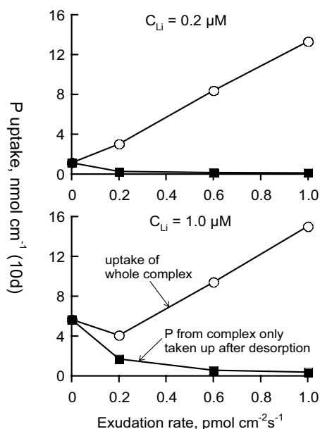
Fig. 1. Phosphorus uptake from a soil of solution concentration (C Li ) of 0.2 μM or 1.0 μM. P is being complexed by root exudates, like citrate, and P uptake is in ionic form from soil solution or after desorption from the complex, or the whole complex is taken up.
