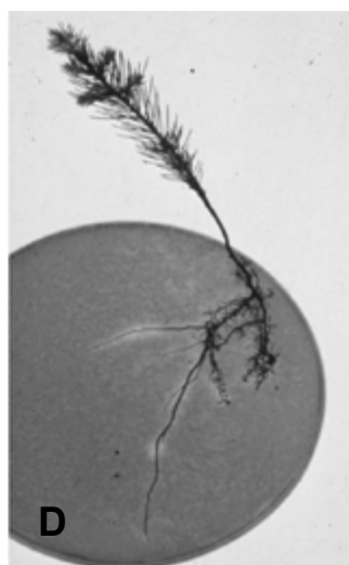
Fig. 1: Principle (A) and applications for in situ detection of Al complexation with the aluminon competition test: (B) Al-complexation along roots of Norway spruce in rhizobox culture. (C) Root-induced Al-complexation in seedlings of Lupinus luteus and (D) Norway spruce, grown in hydroponic culture.
