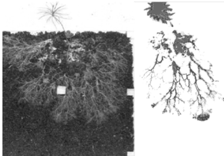
Fig. 1. scan of a microcosm containing a mycorrhizal pine seedling labelled with 14 C CO 2 . The distribution of carbon to the margin of the ectomycorrhizal mycelium is evident (see also colour plate on p. 534).
