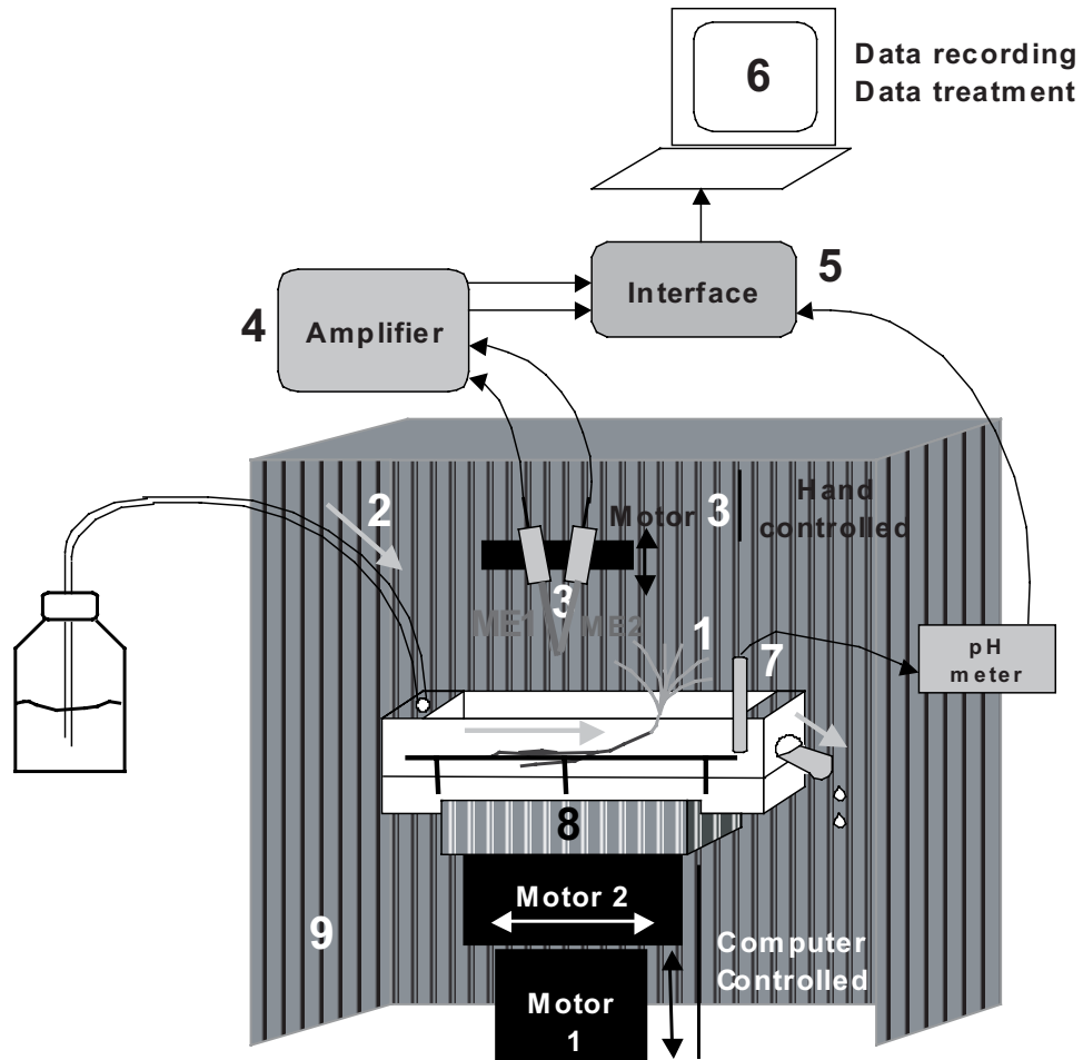
Fig. 1. Experimental set-up for continuous monitoring of ion fluxes using ion-selective microelectrodes. 1: Intact plant in a perspex cuvette, 2: flowing solution, 3: ion-selective microelectrodes plugged in headstages and moved by a hand-controlled motor, 4: amplifier, 5: interface (McLab), 6: computer (MacIntosh), 7: combined pH-macroelectrode, 8: mobile plate moving the cuvette using computer controlled motors, 9: Faraday cage
