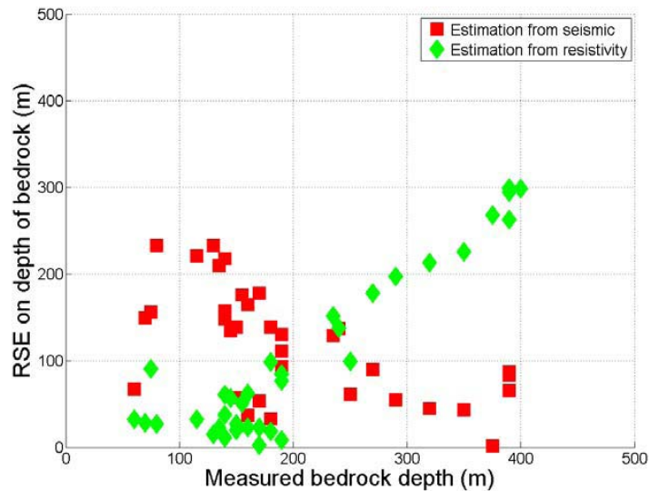
Figure 53: Analysis of RSE of the two methods according to the measured bedrock depth on boreholes
