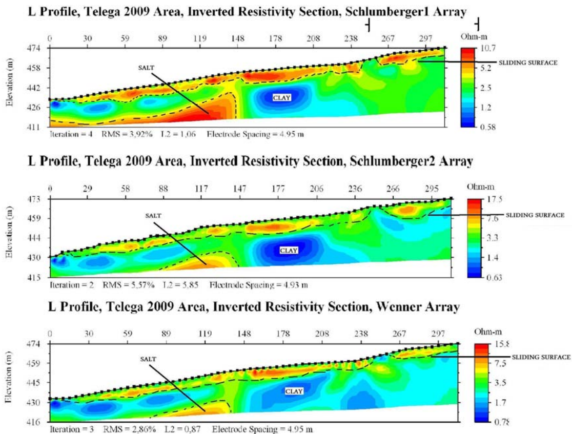
Figure 12: Inverted resistivity section obtained on the longitudinal profile for the Schlumberger1 array, the Schlumberger2 array and the Wenner array
