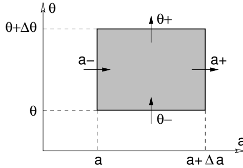
FIGURE 3 – Conservation laws for an infected group of the population dynamics model in space (a, \theta) , with no mortality.
