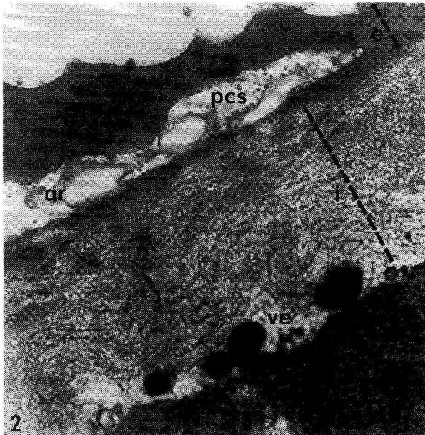
Fig. 2. Pollen wall structure of P. alba . Exine (e): the arcs of the exine (ar) contain pollen coat substances (pcs), likely to be involved in pollen-pistil interactions. Intine (i): osmiophilic vesicles (ve) are observed within the intine. (TEM, x 48 000, uranyl acetate/lead citrate stain).
