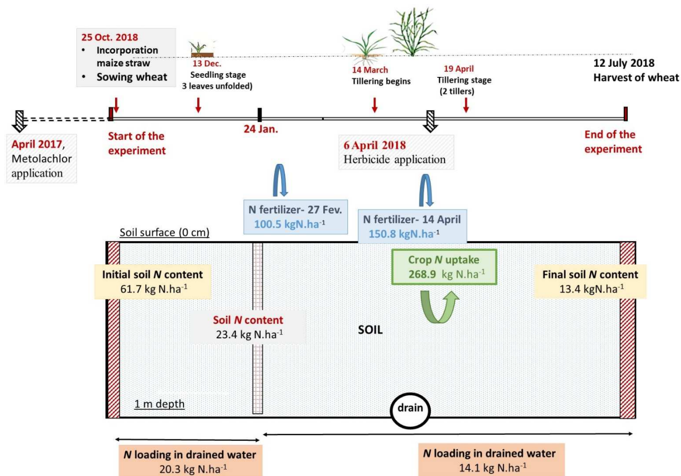
Figure 3. Nitrogen balance (kg N ha -1 ) in the 0–100 cm soil layer, based on the measured values of N fluxes and accounting for mineral N fate at the field site.
