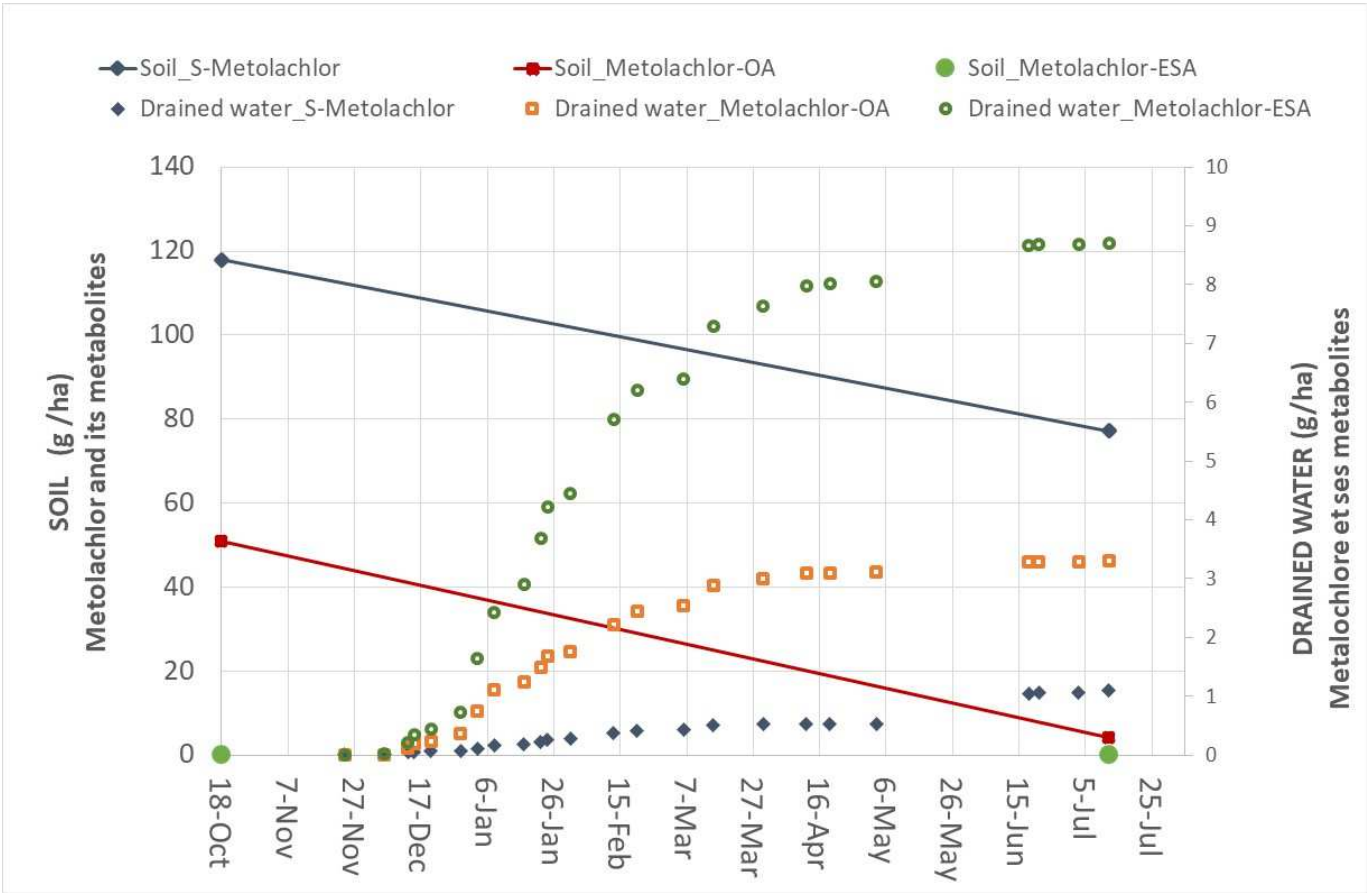
Figure 6. Evolution over time of the amount of S-Metolachlor (cumulative: solid line) and its two metabolites in the soil and drained water
