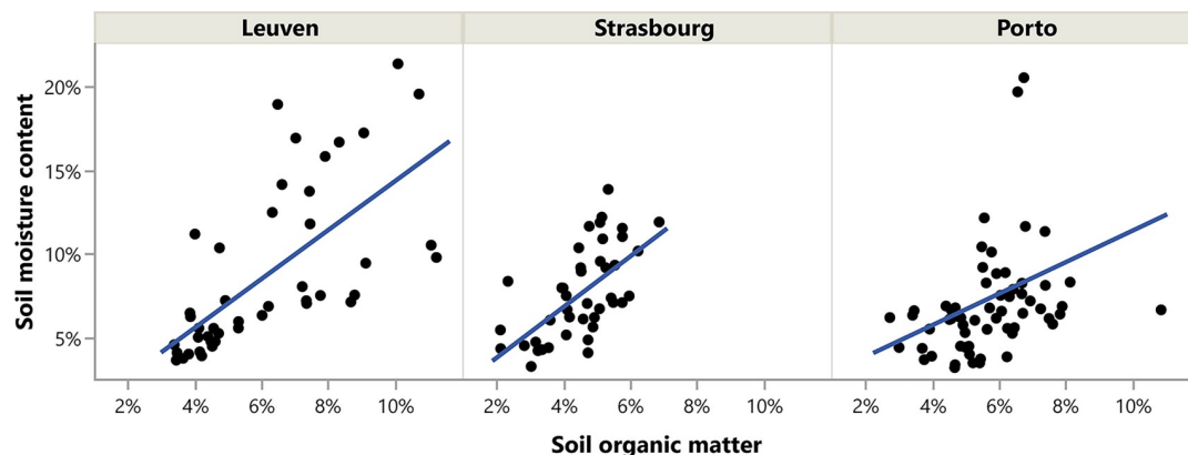
Fig 2. The relation between soil moisture content and soil organic matter in the three sampled cities. A mixed model with moisture content as response variable and soil organic matter as explanatory variable (and city as random factor) showed a strong relation between soil organic matter and soil moisture content ( F = 53.7 , P < 0.001 ).
