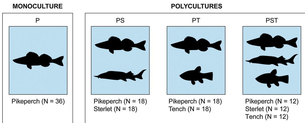
Fig. 1. Description of the experimental design. Four modalities were tested in triplicate: one modality in monoculture: P (pikeperch) and three modalities in polyculture: PS (pikeperch and sterlet), PT (pikeperch and tench) and PST (pikeperch, sterlet and tench). The initial fish number was 36 (with an adjustment of fish number by species according to the modality).
