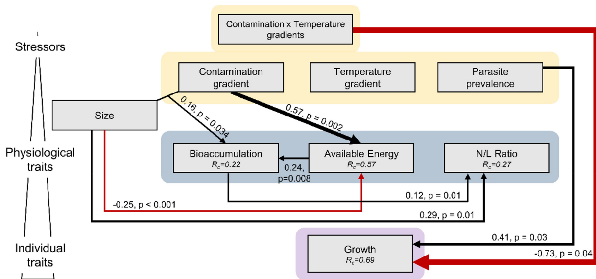
Fig. 3. Structural Equation Models (SEM) testing the effects of stressor gradients on growth and underlying physiological traits (goodness of fit: p = 0.907 , CFI = 2.136, df = 6, n = 197 ). Significant links are represented by solid arrows (red: negative relationship, black: positive relationship). Unstandardized coefficient and p-values are given alongside arrows. Line width represents the strength of the relationship (unstandardized coefficient). (For interpretation of the references to colour in this figure legend, the reader is referred to the web version of this article.)
