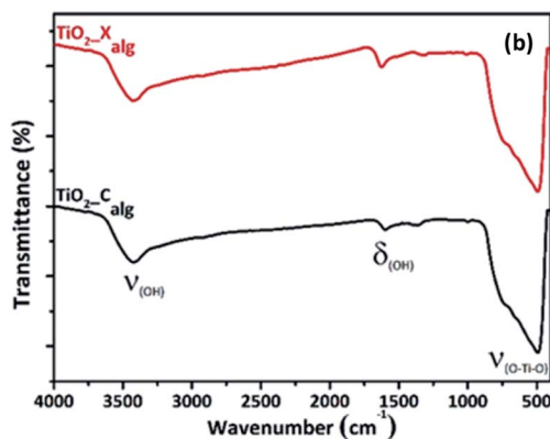
Fig. 6 FTIR spectra of oxides elaborated via the gelation of: (a) CMC and (b) alginate.
