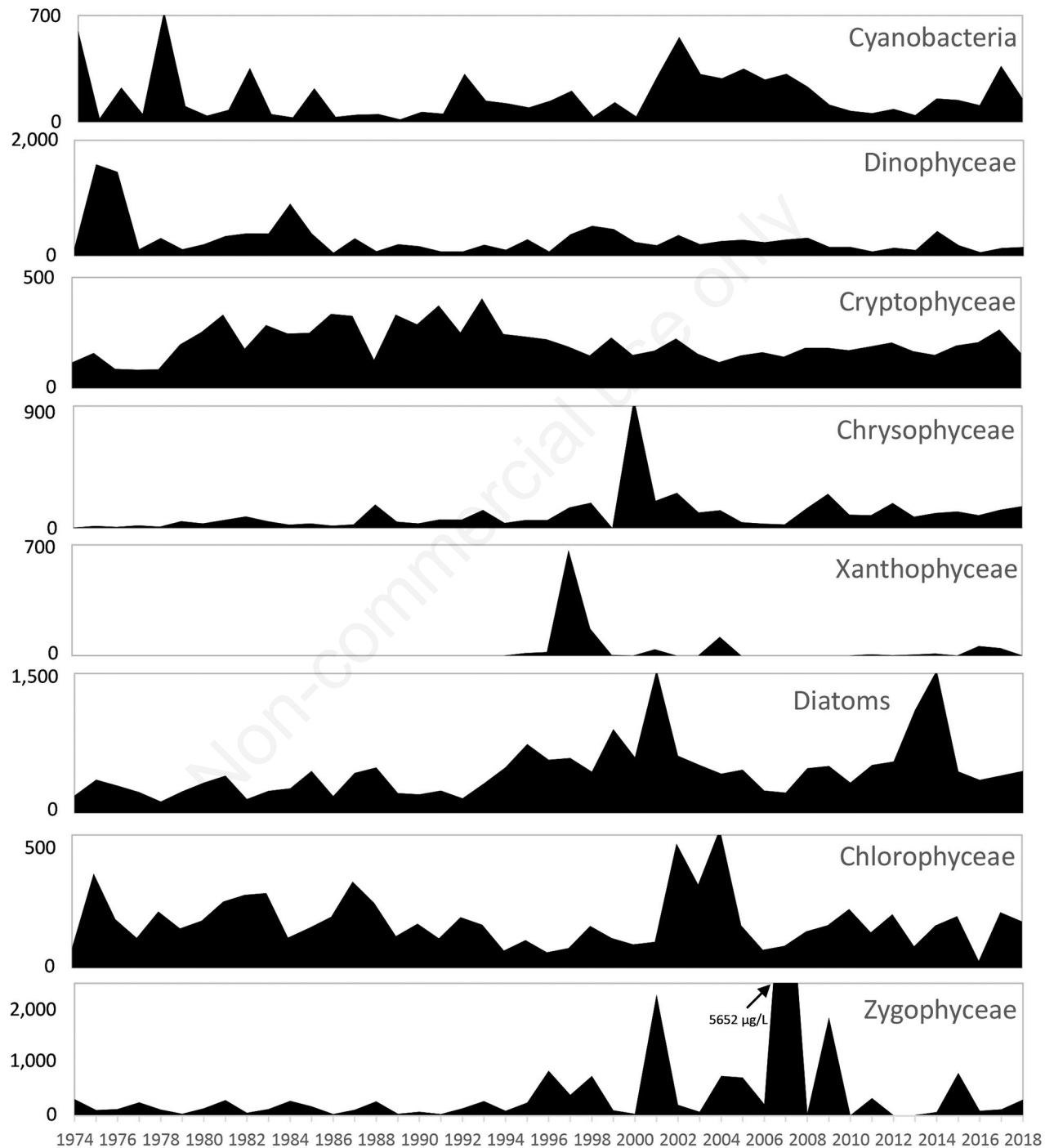
Fig. 5. Taxonomic composition of lake Geneva phytoplankton expressed in biomass (µg/L) from 1974 to 2018 (each value is an annual mean of the water column integrated phytoplankton samplings carried out 2 times a month except once a month between December and February).
