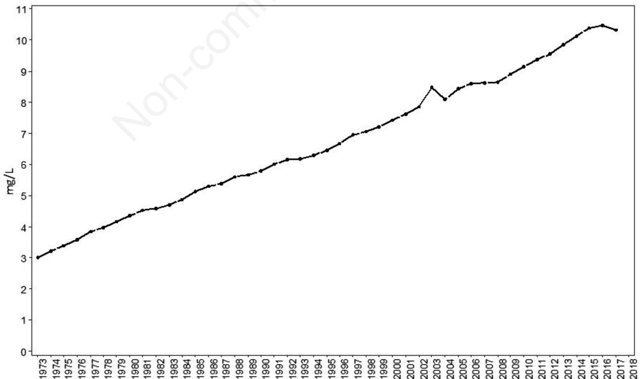
Fig. 3. Interannual dynamic of chlorophyll a in Lake Geneva between 1973 and 2017.
