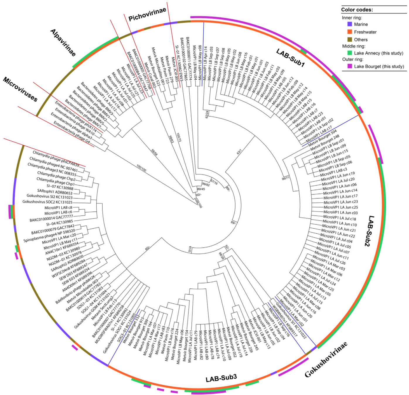
Fig. 1. Bayesian phylogenetic tree based on alignment of 194 homologous amino acid positions of the major capsid protein encoding gene VPI from 167 VPI sequences. Sequences are from lakes Anney and Bourget, Microviridae isolates and other environments (e.g. representative sequences of different defined clusters from other studies). Values at nodes are the Bayesian inference (BI) posterior probabilities and maximum likelihood (ML) bootstrap values (BI/ML). The inner ring represents VPI sequences of the marine field (violet), freshwater (orange) and the others (antique bronze). The middle ring with color strips in green corresponds to sequences from Lake Anney. In the outer ring, sequences labeled with color strips (purple) are from Lake Bourget. “Others” in the color key panel indicates VPI sequences obtained from marine and freshwater sediments, microbialites, sewage water and human gut, mouth, feces or tissue.
