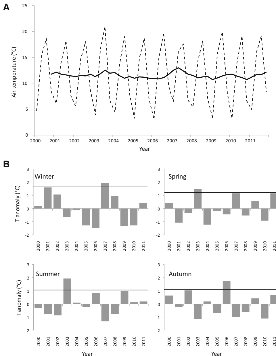
Figure 2. A Long-term changes in seasonal mean air temperature ( dotted line ) and 4-year moving average air temperature ( solid line ). B Long-term changes in seasonal air temperature anomalies measured at the INRA meteorological station from 2000 to 2011. The horizontal line indicates the 99th percentile for seasonal air temperature.
