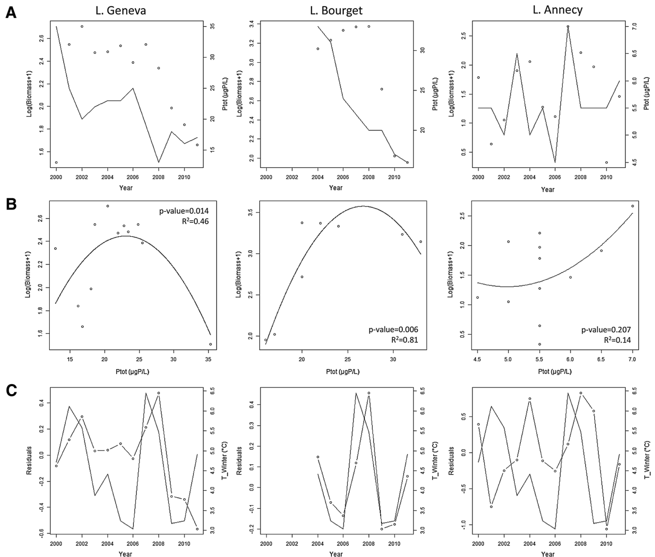
Figure 8. A Long-term changes in cyanobacteria abundance (dots) and total phosphorus concentration measured in February (line). B Relationship between phosphorus and annual cyanobacteria biomass. C Long-term changes in the residuals of the relationship between cyanobacteria and phosphorus (dotted line), and long-term changes in winter water temperature (solid line).
