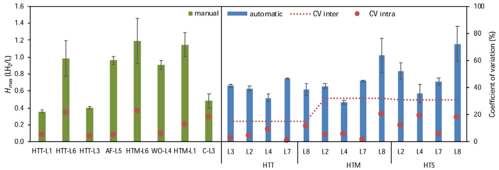
Fig. 7. Cumulative hydrogen production ( H_{max} ) specific to the working volume ( L H_2 L^{-1} ), for the manual and automatic protocols, and its corresponding intra- and inter-laboratory variation. For the manual protocol evaluation different inoculum were tested by different laboratories, meanwhile for the automatic protocol three different source of inoculum were evaluated in different laboratories. The different inoculum sources were heat-treated anaerobic sludge from a thermophilic digester (HTT); heat-treated anaerobic sludge from a mesophilic digester (HTM); biomass from an auto-fermented effluent rich in sucrose (AF); aerobic sludge pretreated by cell wash-out (WO); compost from kitchen wastes (C); and heat-treated anaerobic sludge from a digester treating solid wastes (HTS). L1–L8 stands for results from different laboratories.
