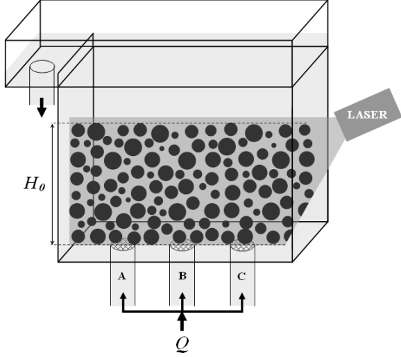
FIG. 1. Schematic of the experimental device. A layer of borosilicate glass beads, of height H_0 , is placed in a rectangular cell of inner section 200 \times 80\text{mm} , previously filled with an oil mixture of the same refractive index as the beads. A fluorescent dye added to the liquid provides a visualization in a vertical slice, within the granular system, by illuminating with a laser sheet. At the bottom of the grain layer, three injection nozzles (ports A, B and C) can be used to generate a localized flow likely to destabilize the medium. The flow rate Q is kept constant and injected by means of a gear pump and the liquid is discharged by overflow, thus maintaining a constant level at the top of the cell.
