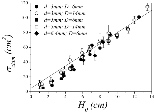
FIG. 8. Critical value of the characteristic section \sigma_{chim} at the onset of fluidized chimney as a function of the initial height H_0 for several experimental series with bead diameter respectively equal to d = 3\text{mm} ( \circ , \bullet ), d = 5\text{mm} ( \square , \blacksquare ), and d = 6.4\text{mm} ( \blacklozenge ), and with two different sizes of the injection hole, D_1 = 6\text{mm} (solid symbols) and D_2 = 14\text{mm} (open symbols). The best fit to Eq.(7) is given by the solid line with \lambda = 24\text{mm} .
