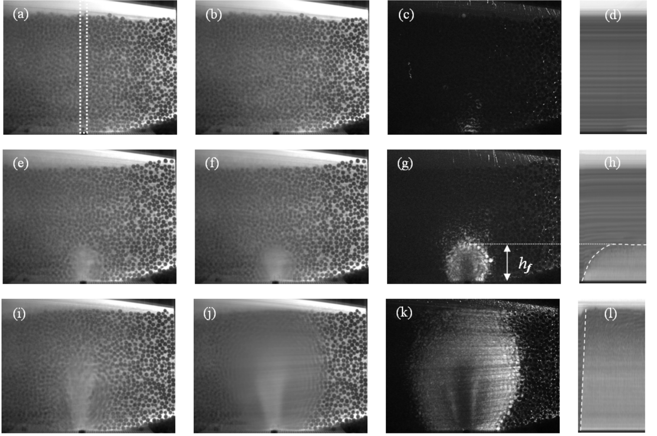
FIG. 2. Illustration of the three different steady states for a 5mm-bead layer of initial height H_0 = 12.0\text{cm} and with an injection hole D_2 = 14\text{mm} : (i) Static regime ( Q = 69.5\text{cm}^3.\text{s}^{-1} ; images a, b, c, and d); (ii) Fluidized cavity regime ( Q = 86.9\text{cm}^3.\text{s}^{-1} ; images e, f, g and h); (iii) Fluidized chimney regime ( Q = 100.8\text{cm}^3.\text{s}^{-1} ; images i, j, k and l). The two first sets of images are respectively an individual picture (images a, e, and i) and the average image (images b, f, and j) in each of the three steady states. The next series of pictures (images c, g, and k) is obtained after subtraction of the average image then projection retaining only the brightest pixels of the entire sequence. The last pictures are spatio-temporal diagrams plotted from the vertical lines centered on the injection hole and contained in the dotted rectangle shown in image a.
