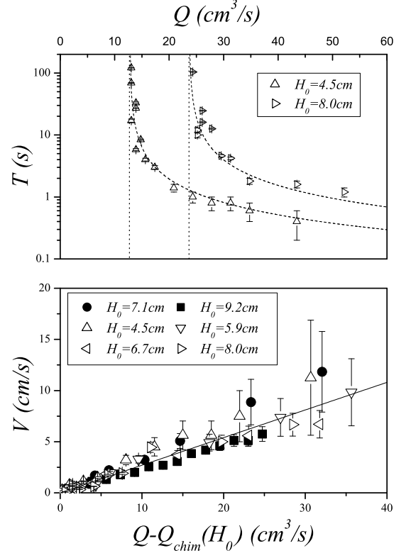
FIG. 6. (Up): Duration T of the upward expansion phase of the fluidized zone, from initiation to establishment of the chimney regime, as a function of flow rate Q with 3mm-beads and injection hole D_2 = 14\text{mm} , and for initial height H_0 = 4.5\text{cm} ( \Delta ) and H_0 = 8.0\text{cm} ( \blacktriangleright ). The vertical dotted lines are the two asymptotes Q = Q_{chim}(H_0) and the dashed curves are of the form: T \propto (Q - Q_{chim})^{-1} . (Down): Global expansion rate V = H_0/T versus excess flow rate Q - Q_{chim}(H_0) with injection holes D_1 = 6\text{mm} (solid symbols) and D_2 = 14\text{mm} (open symbols) and for H_0 = 7.1\text{cm} ( \bullet ), H_0 = 9.2\text{cm} ( \blacksquare ), H_0 = 4.5\text{cm} ( \Delta ), H_0 = 5.9\text{cm} ( \nabla ), H_0 = 4.5\text{cm} ( \triangleleft ), H_0 = 8.0\text{cm} ( \blacktriangleright ). The solid line stands for Eq.(3) with A = 0.27\text{cm}^{-2} .
