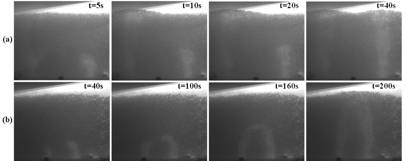
FIG. 7. Successive stages in a sequence of fluidization of a 3mm-beads layer of initial height H_0 = 9.2\text{cm} by two injection holes spaced by \delta and with a constant flow rate Q taken just above the fluidized chimney regime: (a) \delta = \delta_2 = 80\text{mm} and Q = 45.2\text{cm}^3.\text{s}^{-1} ; (b) \delta = \delta_1 = 40\text{mm} and Q = 29.6\text{cm}^3.\text{s}^{-1}
