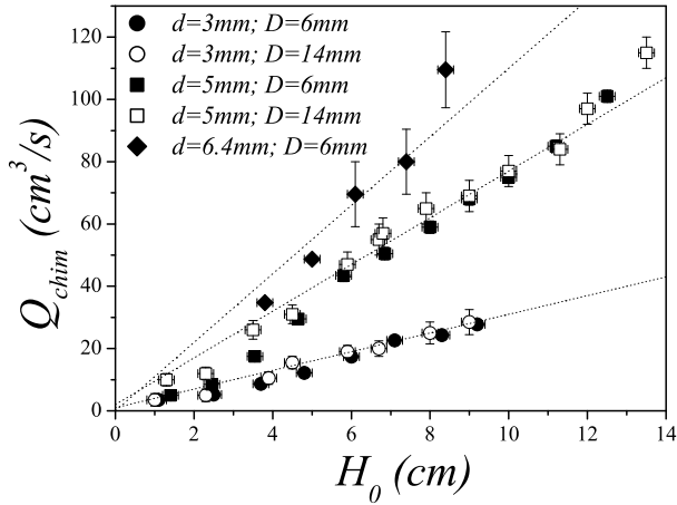
FIG. 5. The critical flow rate Q_{chim} at the onset of fluidized chimney as a function of the initial height H_0 for several experimental series with bead diameter respectively equal to d = 3\text{mm} ( \circ , \bullet ), d = 5\text{mm} ( \square , \blacksquare ), and d = 6.4\text{mm} ( \blacklozenge ), and with two different sizes of the injection hole, D_1 = 6\text{mm} (solid symbols) and D_2 = 14\text{mm} (open symbols). The dotted lines are only guides for the eyes.
