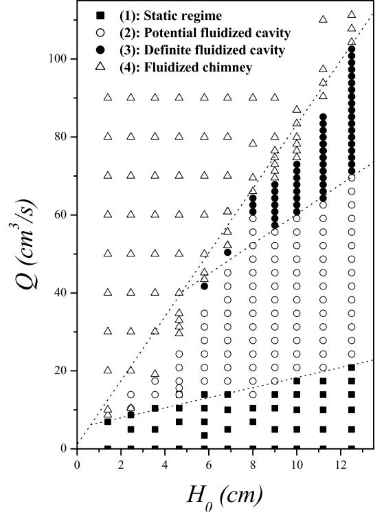
FIG. 4. Phase-diagram summarizing the different steady-states observed when a flow rate Q is injected at the base of a bead layers of initial height H_0 , here with 5mm-beads and an injection hole D_1 = 6\text{mm} . The four regimes are: (1) Static regime (solid square symbols); (2) Potential fluidized cavity regime (open circle symbols); (3) Definite fluidized cavity regime (solid circle symbols); (4) Fluidized chimney regime (open triangle symbols). The dotted lines are only guides for the eyes.
