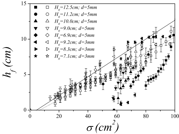
FIG. 9. Height h_f of the fluidized cavity versus \sigma during increasing (solid symbols) and decreasing (open symbols) flow rate sequences for an injection hole D = 6\text{mm} , for two bead diameters ( d = 3\text{mm} and d = 5\text{mm} ) and with several values of the initial height H_0 : d = 5\text{mm} and H_0 = 12.5\text{cm} (square symbols), H_0 = 11.2\text{cm} (circle symbols), H_0 = 10.0\text{cm} (up triangle symbols), H_0 = 9.0\text{cm} (down triangle symbols), H_0 = 6.9\text{cm} (lozenge symbols); d = 3\text{mm} and H_0 = 9.2\text{cm} (left triangle symbols), H_0 = 8.3\text{cm} (right triangle symbols), H_0 = 7.1\text{cm} (diamond symbols). The solid and dotted lines stand for Eq.(8) with respectively \lambda = 24\text{mm} and \lambda = 29\text{mm} .
