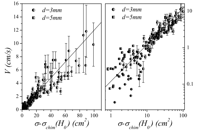
FIG. 10. Expansion rate V = H_0/T plotted versus \sigma - \sigma_{chim}(H_0) in linear-linear and log-log representations for all the data obtained with bead diameters d = 3\text{mm} and d = 5\text{mm} for both injection holes D_1 = 6\text{mm} and D_2 = 14\text{mm} . The solid line stands for Eq.(9) with a = 0.1\text{cm}^{-1}.\text{s}^{-1} .
