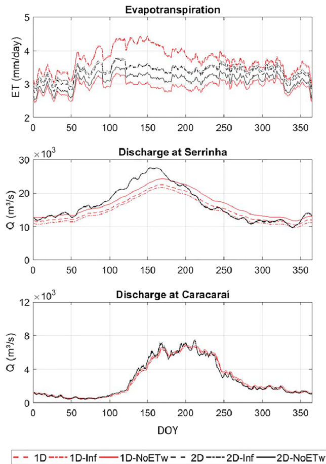
Figure 12. Analysis of the coupling between hydrologic and hydrodynamic processes for simulated evapotranspiration and discharge (Negro River at Serrinha and Branco River at Caracarai) for the scenarios default (with open water evaporation and without infiltration), “Inf” (with infiltration from floodplain into soil), and “NoETw” (without flooded areas open water evaporation).
