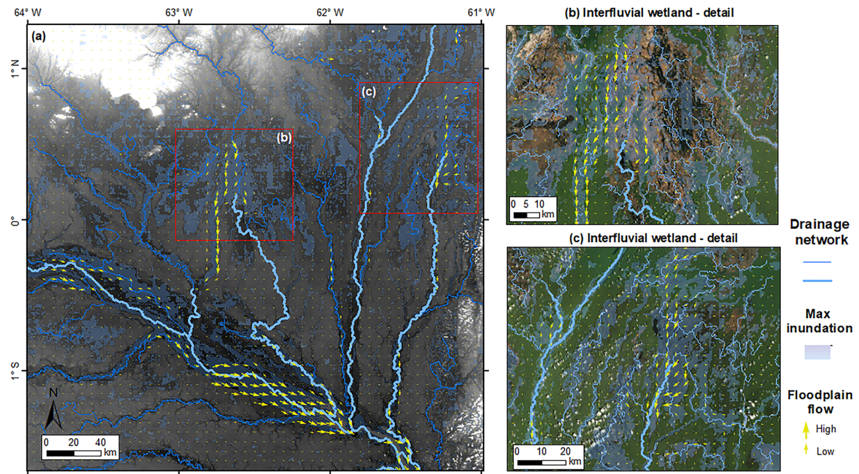
Figure 10. (a) Simulated 2-D floodplain flow direction and magnitude across interfluvial wetlands and Negro mainstem during high water period (19 June 2003). Source of satellite images on panels (b) and (c): Esri, Digital Globe, GeoEye, Earthstar Geographics, CNES/Airbus DS, USDA, USGS, AeroGRID, IGN, and the GIS User Community (Esri, 2009).
