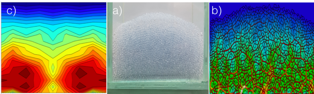
Figure 1. Illustration of the semi-confined heap: experiments and simulations a) experimental device, b) stress field obtained by coarse graining superposed on the force network, c) vertical stress field measured by a local probe.
