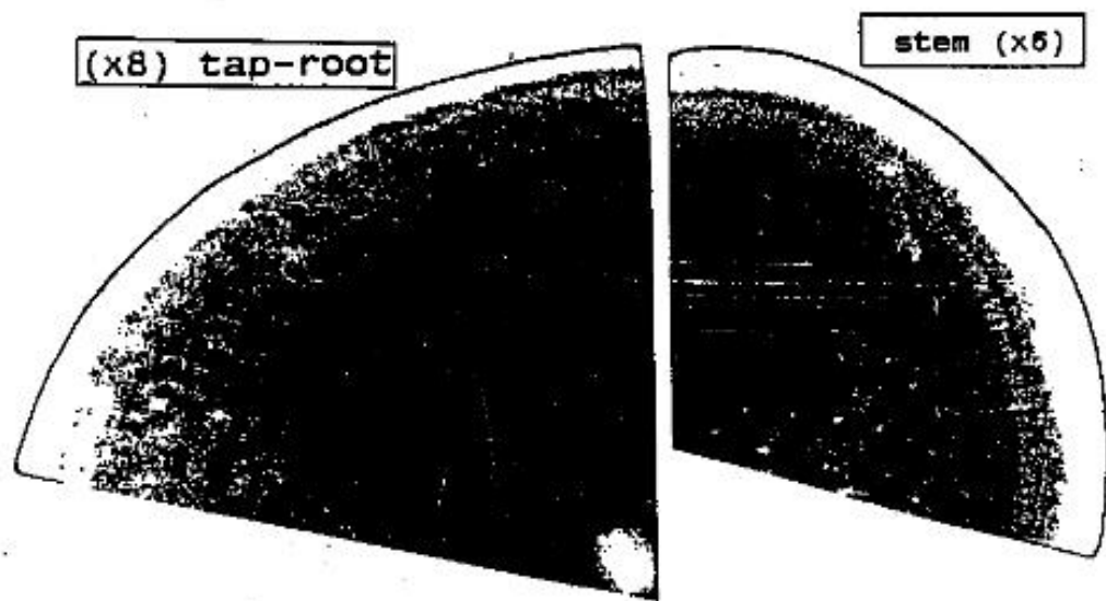
Autoradiographs of wood cross-sections
