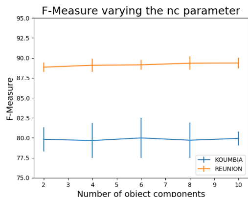
FIGURE 6. The results of the sensitivity analysis of TASSEL regarding the nc parameter on the two real-world benchmarks on the Koumbia and Reunion study sites.
