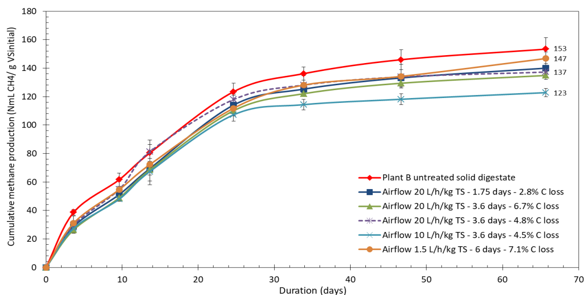
Figure 1 Effects of several short-term aerations on methane potential of plant B solid digestate (mass loss included)
