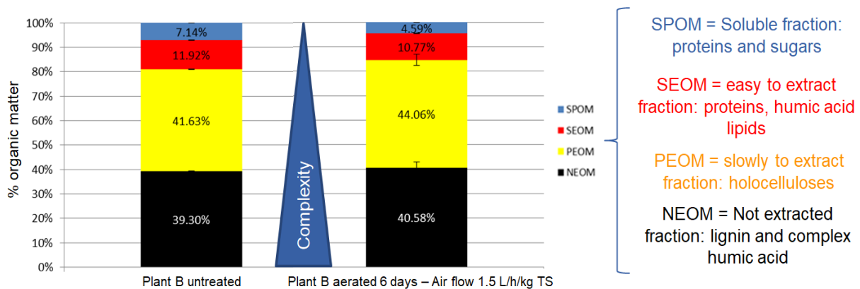
Figure 2 Example of the effect of short term aerobic post-treatment on organic matter bioaccessibility
