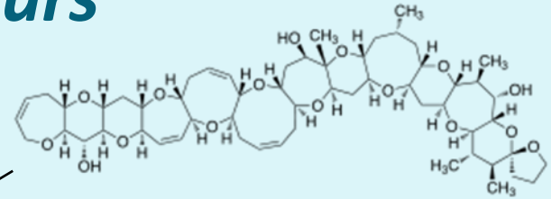
Ciguatoxines
