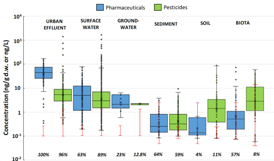
Fig. 4. Level of environmental concentrations and detection frequency of pharmaceutical and pesticidal antifungal azoles in wastewater effluent (n = 46), surface water (n = 154), groundwater (n = 33) sediment (n = 67), soil (n = 15) and biota (biofilms, gammarids, fish) samples (n = 114) in Switzerland. Results are expressed in ng/g d.w. (sediment, soil), ng/g w.w. (biota) or ng/L (urban effluent, surface water, groundwater). The range of LOQs in each compartment is shown in red as detailed in Table S7. The detection frequency in each compartment is expressed as percentage below the graph.
