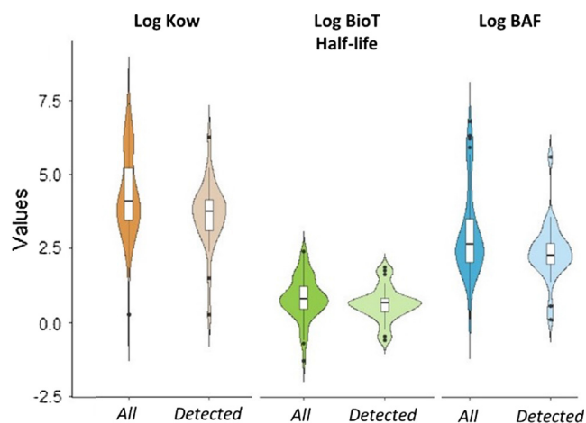
Fig. 3. Physico-chemical ranges of “all” 61 screened and 20 “detected” anti-fungal azoles (From EPISuite v1.4). BioT Half-life is the whole body primary biotransformation rate estimate for fish; BAF is the bioaccumulation factor at the highest trophic level.
