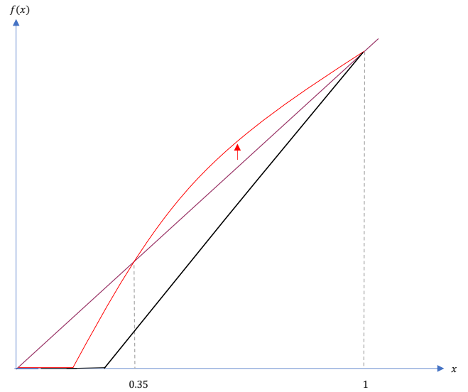
(b) \nu = 0.3, \bar{\theta} = 0.6, \underline{\theta} = 0.4, \tau_p = 0.15
