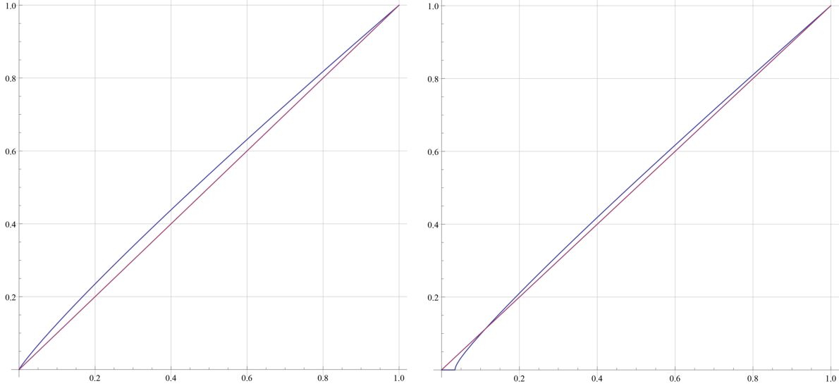
Figure 1: Dynamics for \nu = 0 (left panel) and \nu = 0.1 (right panel), with x_t on the X-axis and x_{t+1} on the Y-axis. The blue curve is the dynamic equation characterizing equilibrium paths x_{t+1} = f(x_t) , while the pink curve is the first bisector x_{t+1} = x_t .
