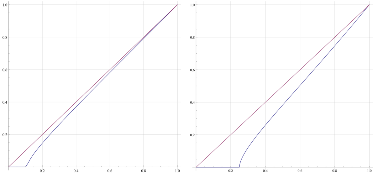
Figure 2: Dynamics for \nu = 0.3 (left panel) and \nu = 0.6 (right panel), with x_t on the X-axis and x_{t+1} on the Y-axis. The blue curve is the dynamic equation characterizing equilibrium paths x_{t+1} = f(x_t) , while the pink curve is the first bisector x_{t+1} = x_t .
