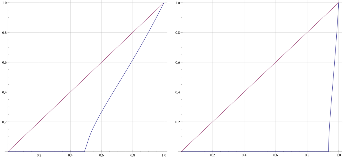
Figure 3: Dynamics for \nu = 1 (left panel) and \nu = 1.45 (right panel), with x_t on the X-axis and x_{t+1} on the Y-axis. The blue curve is the dynamic equation characterizing equilibrium paths x_{t+1} = f(x_t) , while the pink curve is the first bisector x_{t+1} = x_t .
