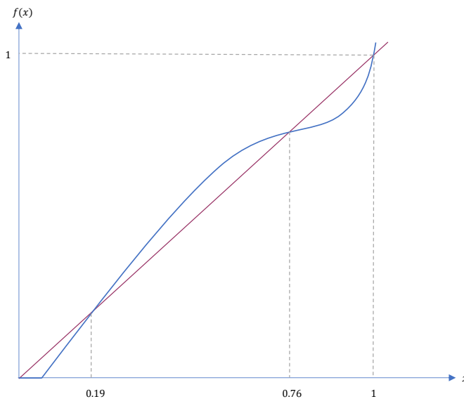
Figure 4: Dynamics for the calibrated values summarized in Table 1 and \xi = 0.8 and \nu = 0.23 .
