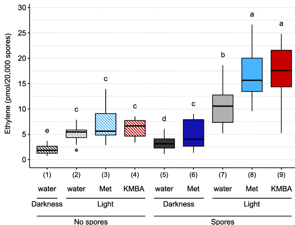
Fig 3. Ethylene production by R. irregularis in response to different treatments. 20,000 spores were germinated for three days in the dark, in the presence or absence of 10 mM methionine (Met) or 1 \mu M \alpha -keto \gamma -methylthio butyric acid (KMBA). Tubes were then sealed with a gas-tight stopper and exposed to light or darkness for 24h. One mL of the headspace gas was then analysed by gas chromatography. Different letters indicate different statistical groups (pairwise Kruskal-Wallis test with FDR correction, P < 0.05 ).
