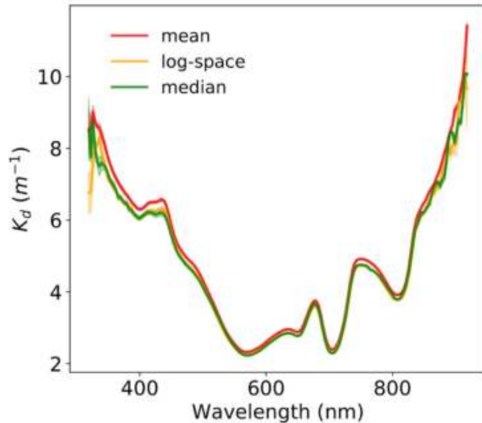
In-Water Radiometry
