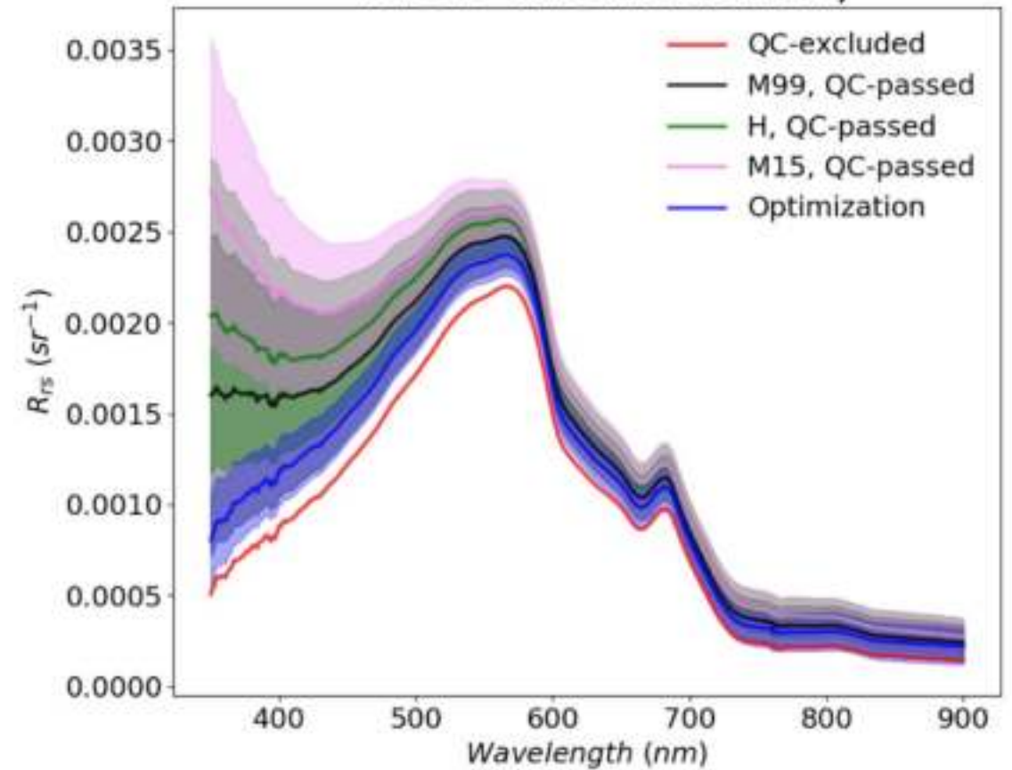
Above-Water Radiometry
