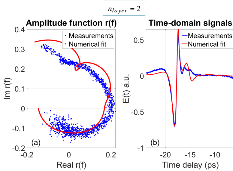
Fig. 13. (a) numerical fit of the Fourier amplitude signal plotted in the complex plane for a 2-layer stack. (b) is a time-domain reconstruction by inverse Fourier transform.
