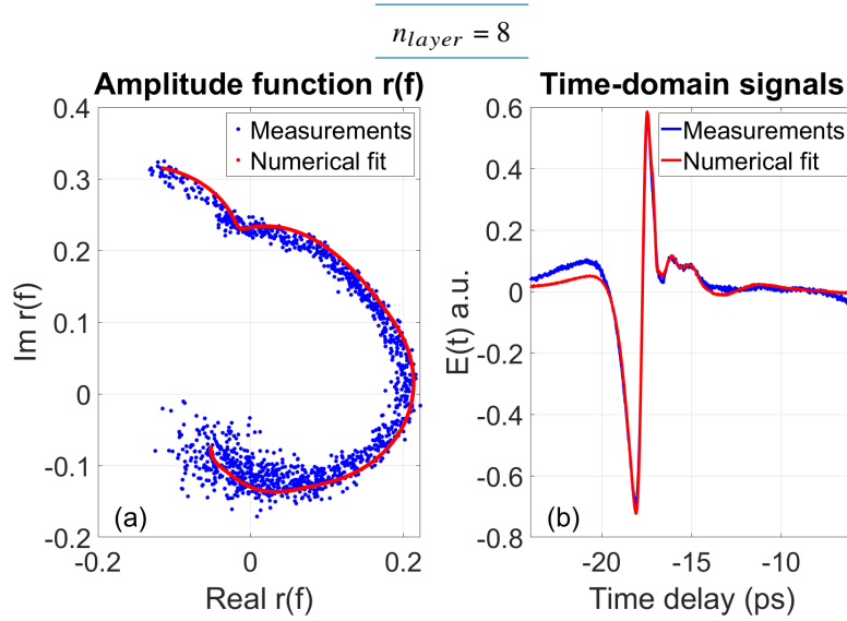
Fig. 14. (a) numerical fit of the Fourier amplitude signal plotted in the complex plane for a 8-layer stack. (b) is a time-domain reconstruction by inverse Fourier transform.
