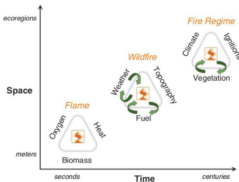
Figure 2 : Controls on fire at different scales of space and time. This framework adds a fire regime triangle (upper right) to the traditional triangles used to characterize combustion (lower left) and the fire environment (middle). Arrows represent feedbacks between fire and the forces controlling fire at different scales.
