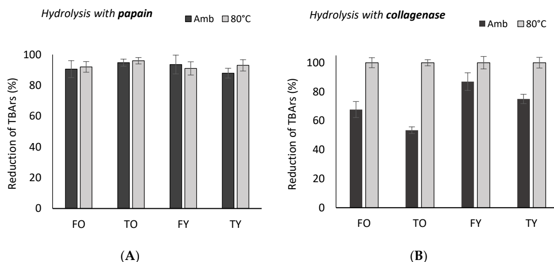
Figure 7. Reduction of TBARs (%) in bovine meat (semimembranosus muscle) at ambient temperature and at 80 °C through the addition of collagen peptides solutions (<3000 Da) from young and old bovine femur and tibia obtained through the enzymes papain (A) and collagenase (B). FO = old femur, 10 years; TO = old tibia, 10 years; FY = young femur, 4.5 years; TY = young tibia, 4.5 years.
