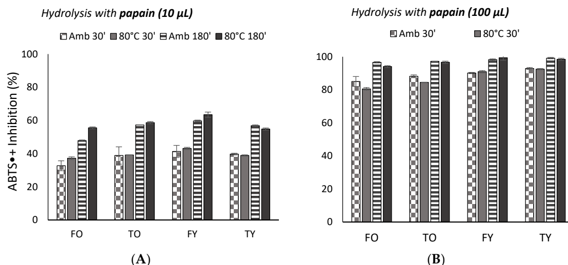
Figure 5. ABTS•+ inhibition (%) by collagen peptides solutions (<3000 Da) obtained through the most effective enzyme, i.e., papain, for 10 µL (A) and 100 µL peptides solutions (B), at ambient temperature and 80 °C, and after 30 and 180 min of incubation. FO = old femur, 10 years; TO = old tibia, 10 years; FY = young femur, 4.5 years; TY = young tibia, 4.5 years.
