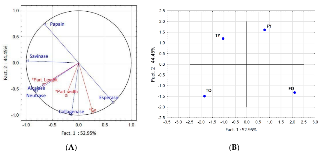
Figure 2. Principal component analysis (PCA) on collagen peptides concentration considering enzymes and particle size as variables (A: loading plot) and bone age and anatomy as individuals (B: score plot). FO = old femur, 10 years; TO = old tibia, 10 years; FY = young femur, 4.5 years; TY = young tibia, 4.5 years.
