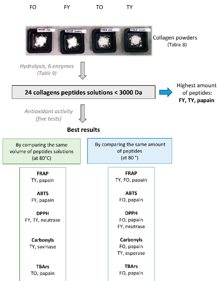
Figure 10. Overview of the antioxidant activity of bovine bone collagen peptides (at 80 °C) by considering bones of different ages and anatomies (femur old, 10 and; femur young, 4.5 years; tibia old, 10 years; tibia young, 4.5 years), and six enzymes (alcalase, collagenase, esperase, neutrased, papain, savinase).
