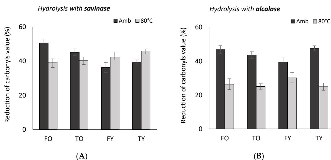
Figure 6. Reduction of carbonyls value (%) in bovine meat (semimembranosus muscle) at ambient temperature and at 80 °C through the addition of collagen peptides solutions (<3000 Da) from young and old bovine femur and tibia obtained through the enzymes savinase (A) and alcalase (B). FO = old femur, 10 years; TO = old tibia, 10 years; FY = young femur, 4.5 years; TY = young tibia, 4.5 years.
