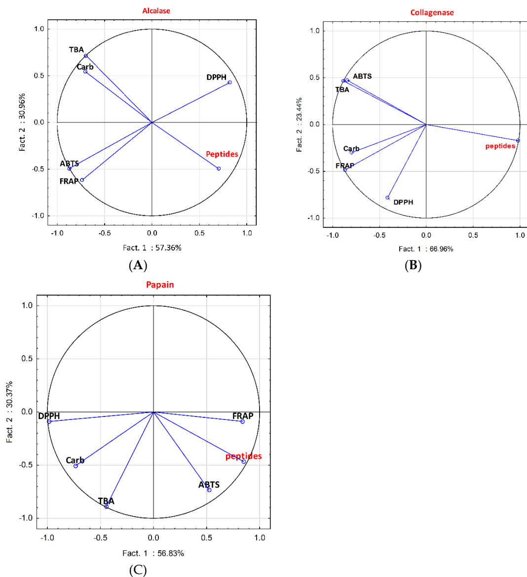
Figure 8. PCA loading plot of antioxidants activity and peptides concentration for alcalase (A), collagenase (B) and papain (C).
