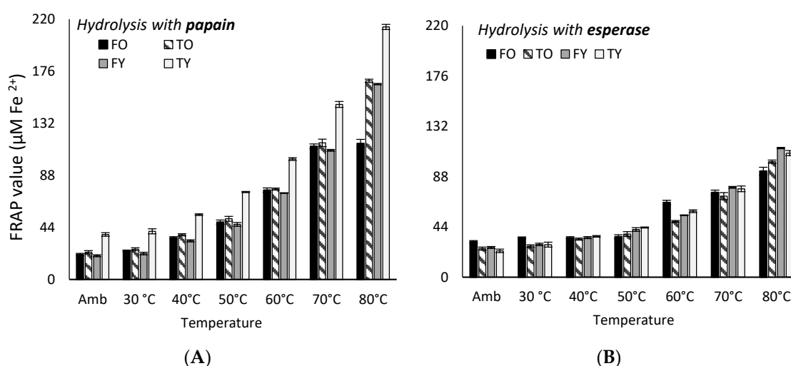
Figure 3. Highest (A) and lowest (B) FRAP values ( \mu\text{M Fe}^{2+} ) for collagen peptides solutions (<3000 Da) obtained through papain and esperase, respectively, at increasing temperatures. FO = old femur, 10 years; TO = old tibia, 10 years; FY = young femur, 4.5 years; TY = young tibia, 4.5 years.
