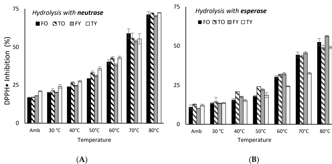
Figure 4. Highest and lowest DPPH• inhibition (%) for collagen peptides solutions (<3000 Da) obtained through neutrase (A) and esperase (B), respectively, and at increasing temperatures. FO = old femur, 10 years; TO = old tibia, 10 years; FY = young femur, 4.5 years; TY = young tibia, 4.5 years.
