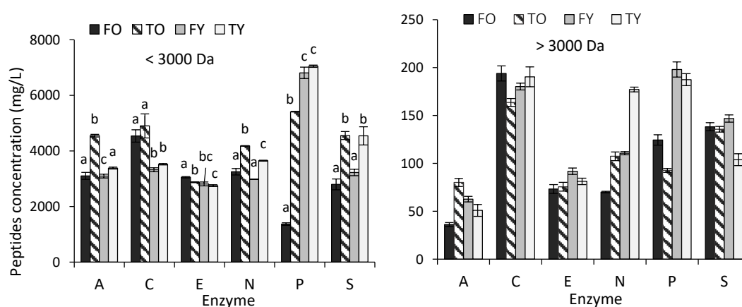
Figure 1. Concentration of peptides, <3000 Da (left) and >3000 Da (right) (equivalents of collagen, mg/L) from young and old bovine femur and tibia collagen solutions hydrolysed through the enzymes alcalase (A), collagenase (C), esperase (E), neutrase (N), papain (P), savinase (S) (mean values \pm standard deviation (SD), n = 3 ). For each enzyme, significant differences among bones ( p < 0.05 ) are indicated by different lowercase letters (only for the left Figure). FO = old femur, 10 years; TO = old tibia, 10 years; FY = young femur, 4.5 years; TY = young tibia, 4.5 years.
