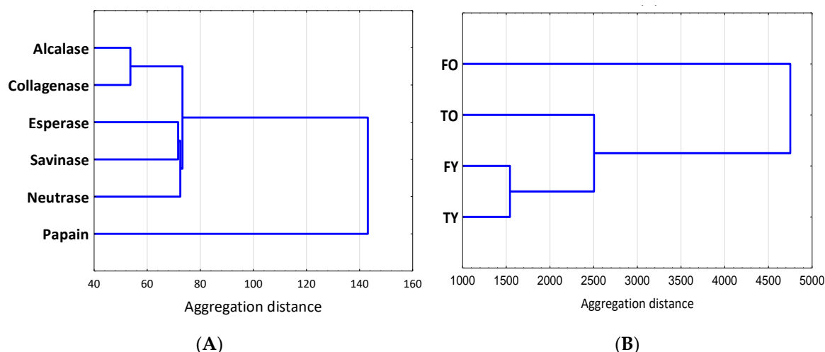
Figure 9. (A) Hierarchical clustering analysis (HCA) of enzymes on the basis of the antioxidant activities and for all the bones (FO, TO, FY and TY); (B) HCA of bones based on antioxidants activities and amount of peptides released by each enzyme. FO = old femur, 10 years; TO = old tibia, 10 years; FY = young femur, 4.5 years; TY = young tibia, 4.5 years.
