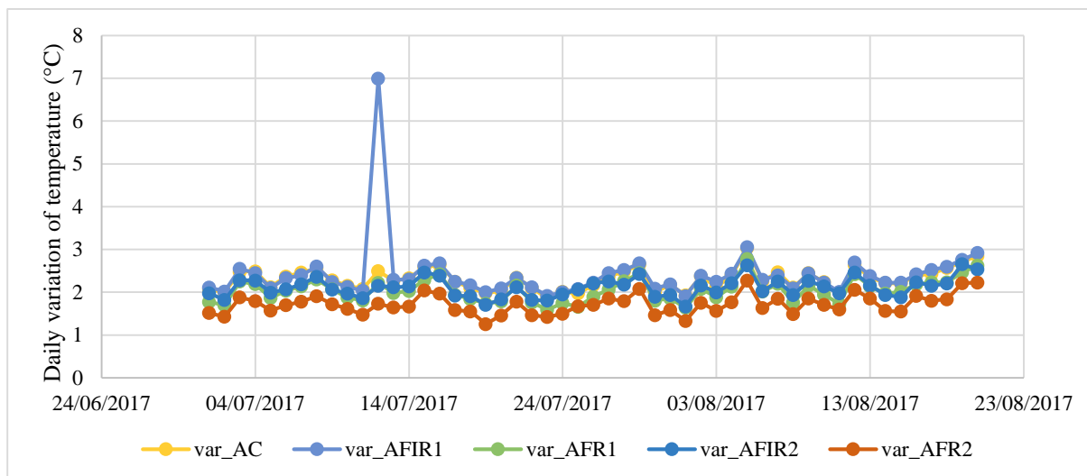
Figure 26: Daily variation of temperature recorded by HMP155 sensors on the plot A1 from the domaine de Restinclières recorded from the 1 st of July 2017 to the 20 th of August 2017. There are 5 sensors on the plot, one the open is the control (AC) and the four others are in each agroforestry modality and in the 2 different blocks (AFIR1/AFR1; AFIR2/AFR2) with AFIR: Agroforestry inter-row and AFR: Agroforestry row.
