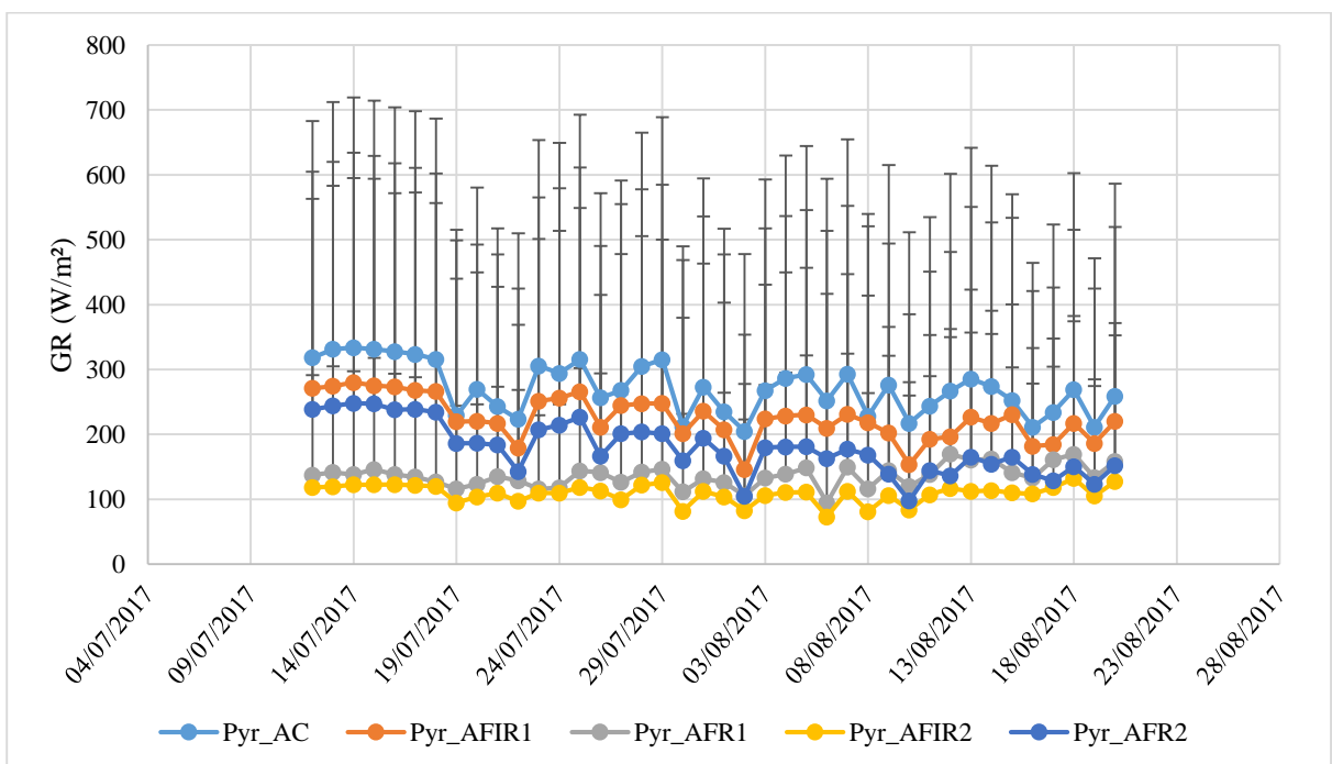
Figure 11: Daily average global radiation (mean \pm SD) recorded by SP1110 pyranometers on the plot A1 from the domaine de Restinclières recorded from the 12 th of July 2017 to the 20 th of August 2017. There are 5 pyranometers on the plot, one the open is the control (AC) and the four others are in each agroforestry modality and in the 2 different blocks (AFIR1/AFR1; AFIR2/AFR2) with AFIR: Agroforestry inter-row and AFR: Agroforestry row.
