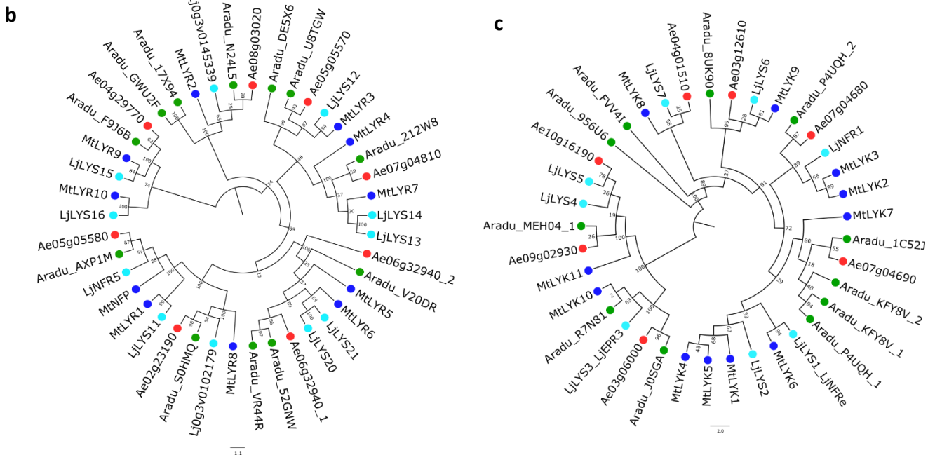
Fig. 2 Comparative analysis of symbiotic receptors, signaling and infection genes
