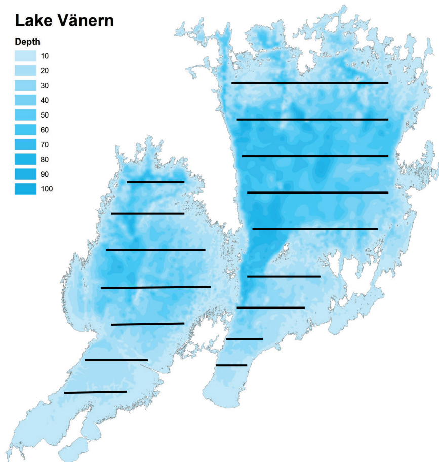
Survey design - 300 km of parallel hydroacoustic transects covering 4 500 km 2 of pelagic area in Lake Vänern (Sweden) result in an acceptable pre-planned coverage (Aglen 1983). Analyses of survey results may result in adaptations of the initial survey design.
