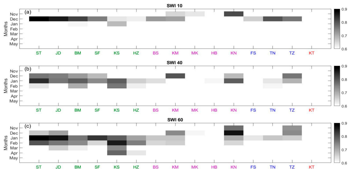
Figure 5. Correlation between the SWI 10 (a), SWI 40 (b), SWI 60 (c) and cereal yield at the province scale: Settat, JD: El Jadida, BM: Beni Mellal, SF: Safi, KS: Kelaa des Sraghna, HZ: Haouz, BS: Ben Slimane, KM: Khemisset, MK: Meknes, HB: El Hajeb, KN: Khenifra, FS: Fes, TN: Taounat, TZ: Taza, KT: Kenitra. All the correlations are significant at the 99% level.
