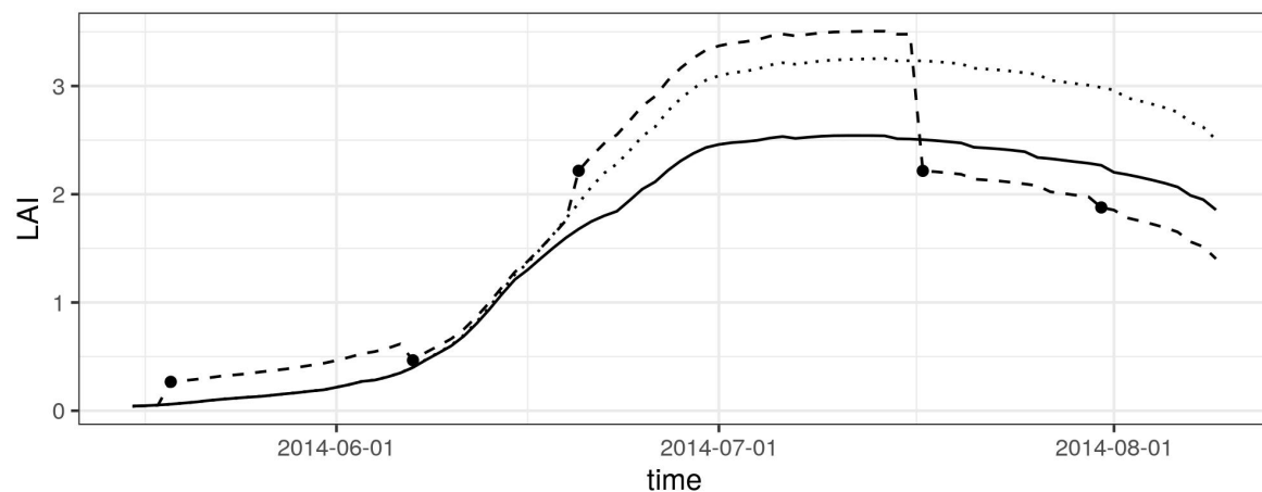
Figure 4. Open-loop simulation, direct insertion (DI) and least square estimator (LSE) illustrated on a plot of this study. Daily LAI values from observations (dots), open-loop (dotted line), DI (dashed line) and LSE (solid line) are plotted from the sowing day to the day of forecast.
