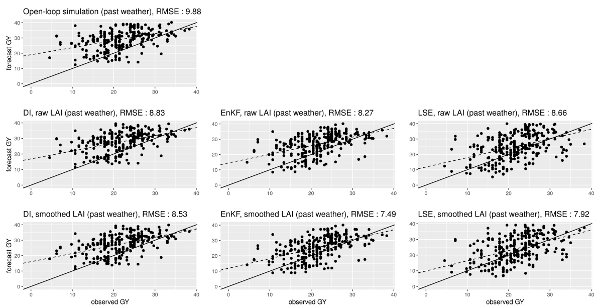
Figure 8. Forecast grain yields (GY) as a function of observed yield. Forecast and RMSE value for the open-loop simulation method (first line), the three assimilation methods (respectively DI, EnKF, LSE) based on raw LAI (second line) and the same three methods based on smoothed LAI (third line). The black solid line represents 1:1 line.
