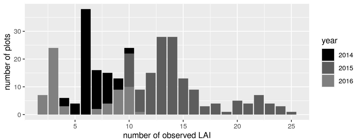
Figure 3. The 281 plots of the field network distributed according to the year and the number of available LAI observations during the period May–August.
