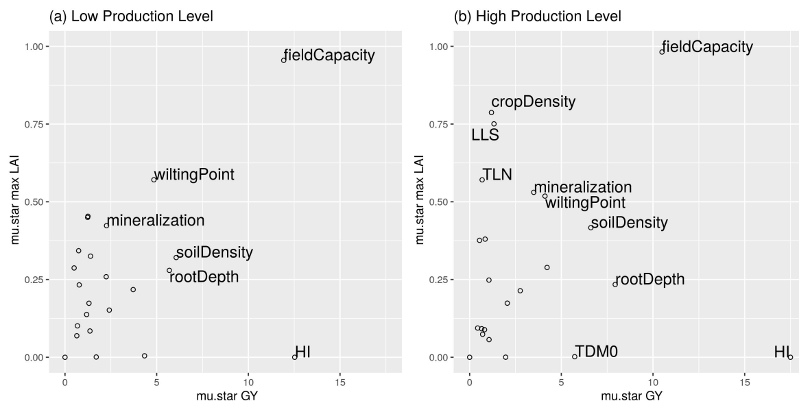
Figure 7. Means of absolute elementary effects ( \mu_{\text{star}} ) computed by the Morris method for two contrasted production situations and for two model outputs: grain yield (GY) and maximal LAI.
