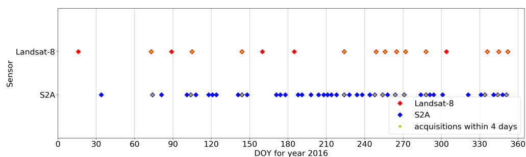
Figure 1. Acquisition dates in day of year (DOY) from Sentinel-2A and Landsat-8 for the year 2016.
