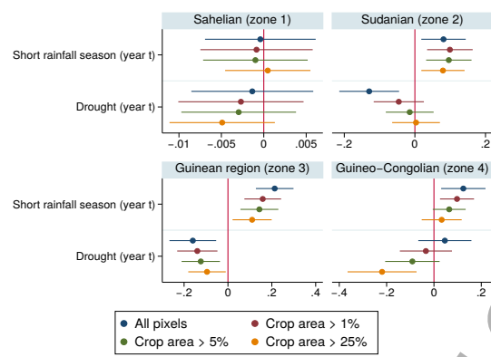
Figure 12: Impact of a bad rainy season on deforestation ( threshold: 25% of canopy cover).
