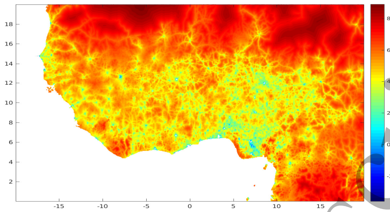
Figure 9: Log time-distance (minutes) to cities in 2015 (of pixels of 1500 inhabitants per km 2 , initial resolution: 1 km).
