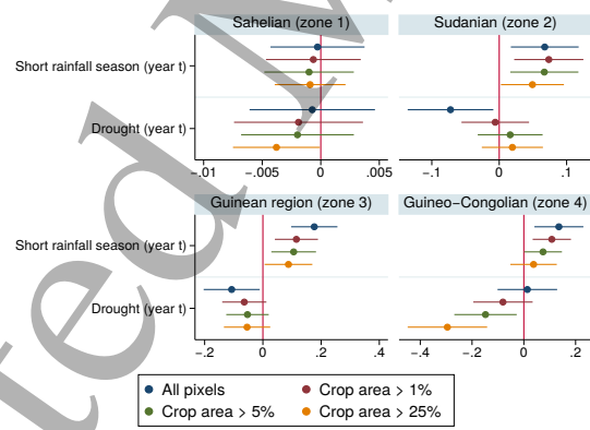
Figure 13: Impact of a bad rainy season on deforestation ( threshold: 30% of canopy cover).
