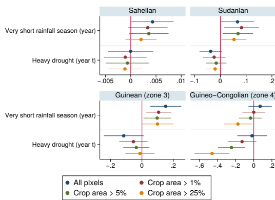
Figure 16: Impact of a very bad rainy season on deforestation (heavy droughts and very short rainy seasons, both defined by SPI inferior to -1.5 ).
