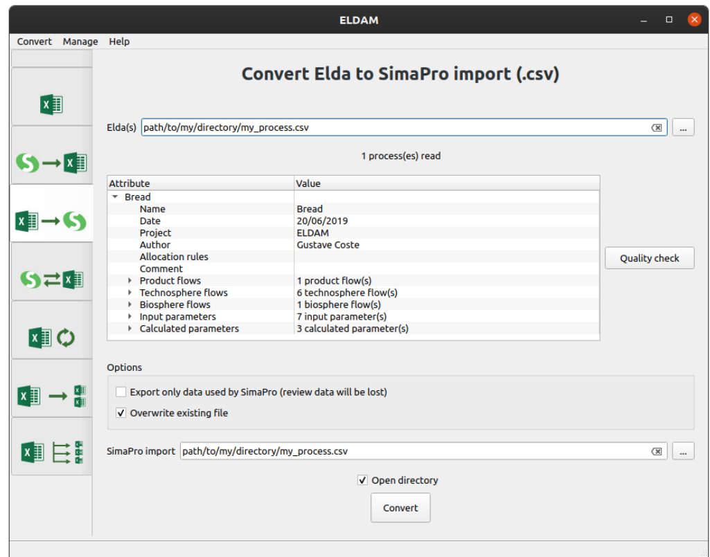
Figure 2: ELDAM's GUI.
