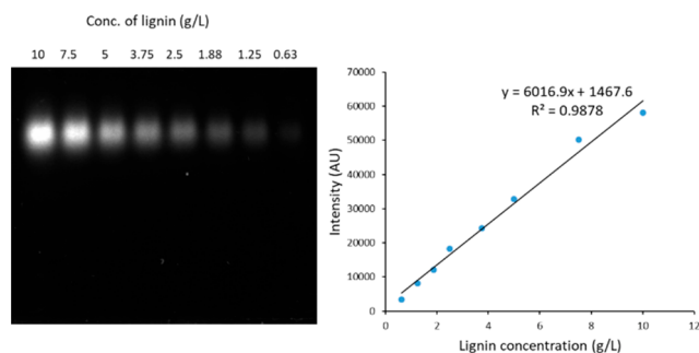
Figure 4. Serially diluted Kraft lignin KL1 run on a 1% agarose gel at pH 8.8, 50 V, for 60 min, and calibration curve with points taken from [Image] fluorescence maxima in each lane.
