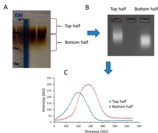
Figure 2. (A) Visible light image of minigel with Kraft KL1 lignin samples run under preferred conditions and ruler with millimeter graduations. (B) Second gel run with lignin extracted from the top half and bottom half of the band shown. (C) ImageJ trace of gel B showing fluorescence intensity vs migrating distance (arbitrary units) of lanes 1 (blue), 2 (empty), and 3 (red).
