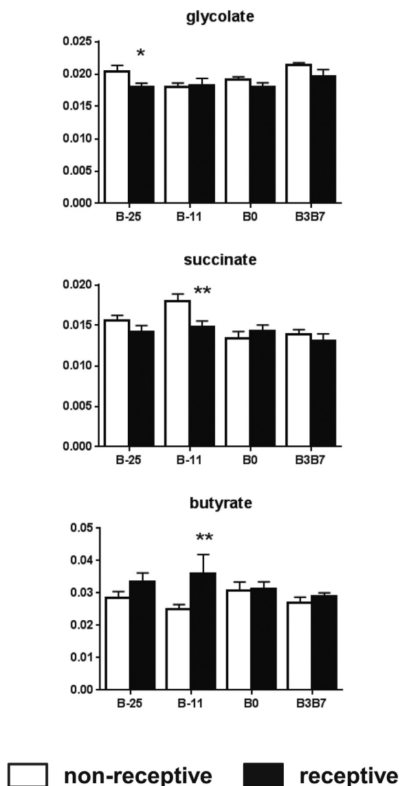
Fig. 4. ^1\text{H} nuclear magnetic resonance spectroscopy analysis of the concentrations of glycolate, succinate, and butyrate (arbitrary unit \pm SEM) in saliva of receptive and non-receptive gilts collected 25 days and 11 days before boar introduction (B-25 and B-11), the day of boar introduction (B0), 3 days later for receptive gilts (B3), or 7 days later for non-receptive gilts (B7). For each metabolite, the y-axis was standardized to the maximal concentration, so that the variations are easy-to-read. * and **: statistical differences between receptive and non-receptive gilts for each collection day, P < 0.05 and P < 0.01 .
