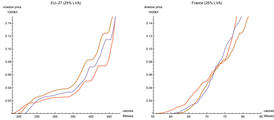
Figure 2. Shadow prices associated with food calorie production when varying at the EU level (left) and the France level (right) - Focus when shadow price lower than 1\text{€}/\text{kg}_{sweq} for the years: — 2010 — 2011 — 2012.
