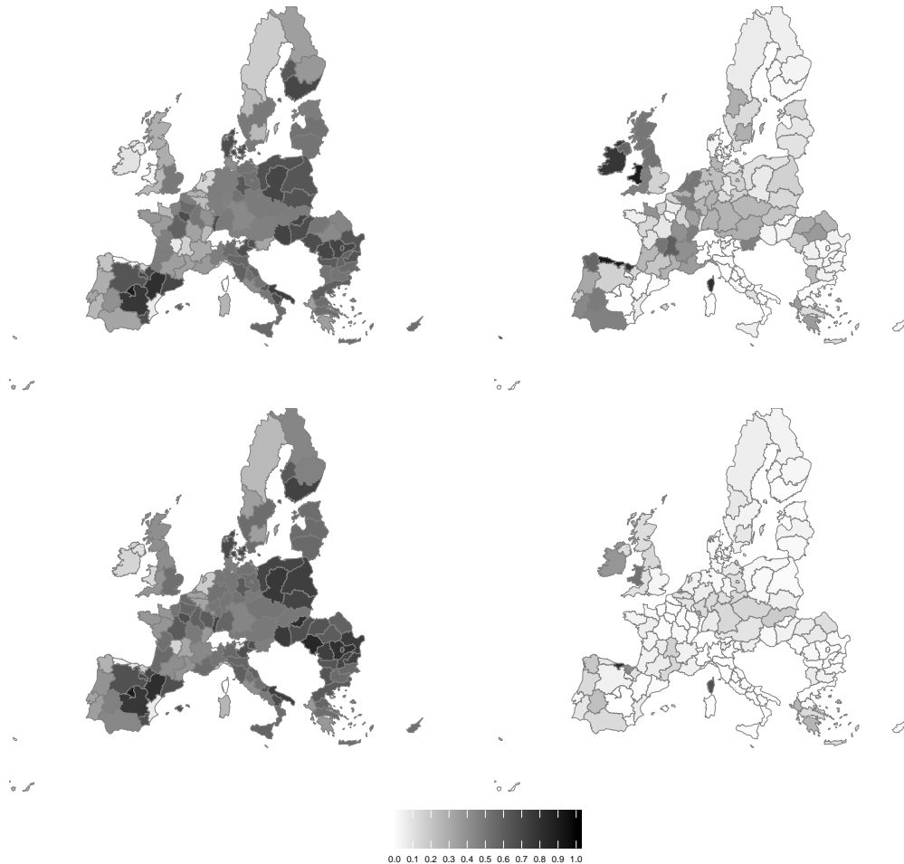
Figure 6. Change in regional average share of the area dedicated to cereals (left) and grasslands (right) from 2012-based starting situation providing 200Mt sweq (top) to the 2012-based situation with production of 500Mt sweq (bottom).
