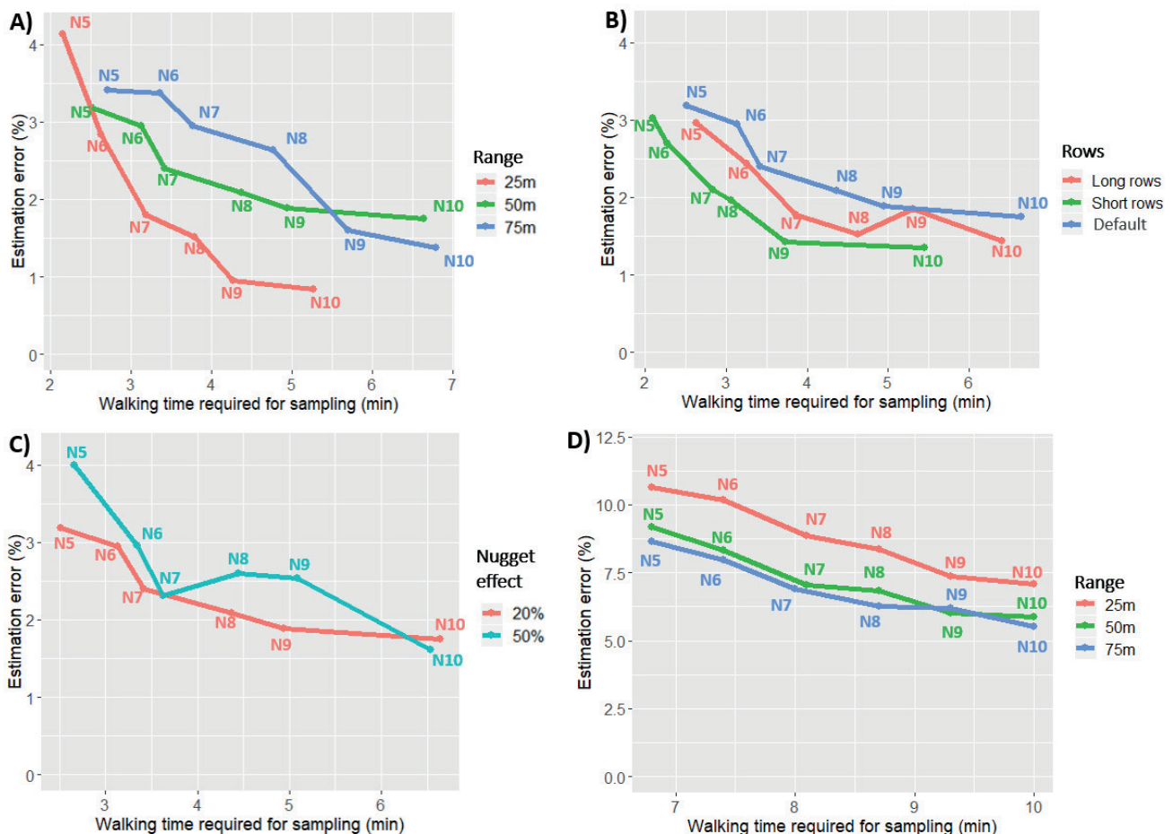
FIGURE 1. Average estimation error and walking times depending on field characteristics: A) the field range, B) row length, C) percentage of random variability (nugget effect). Results are the mean value over ten simulations. Each curve is made of 6 points corresponding to sampling routes with N = \{5, 6, 7, 8, 9, 10\} sampling sites. D) gives the same result as A) but for random sampling and results are the mean value over ten simulations and 100 repetitions per simulation.
