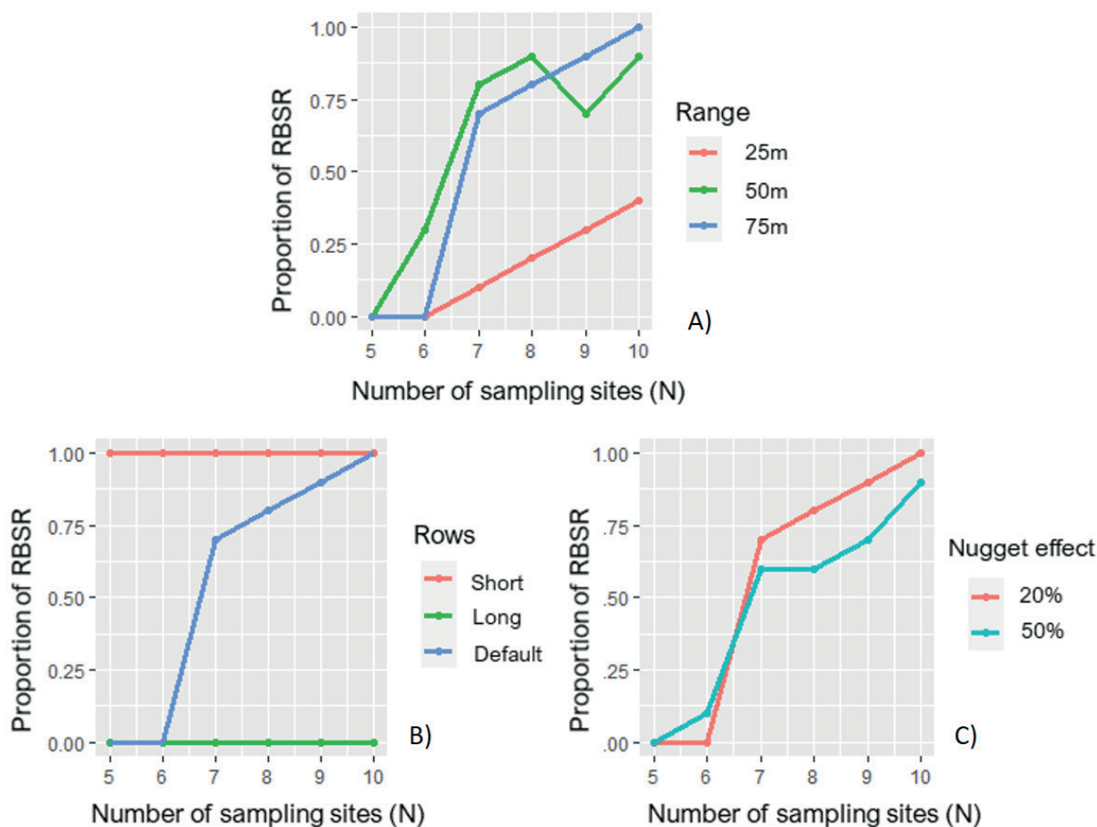
FIGURE 5. Proportion of RBSR sampling strategies sampling route depending on the number of sampling sites (N) and field type (A) range, B) row length of the field and C) nugget effect).
