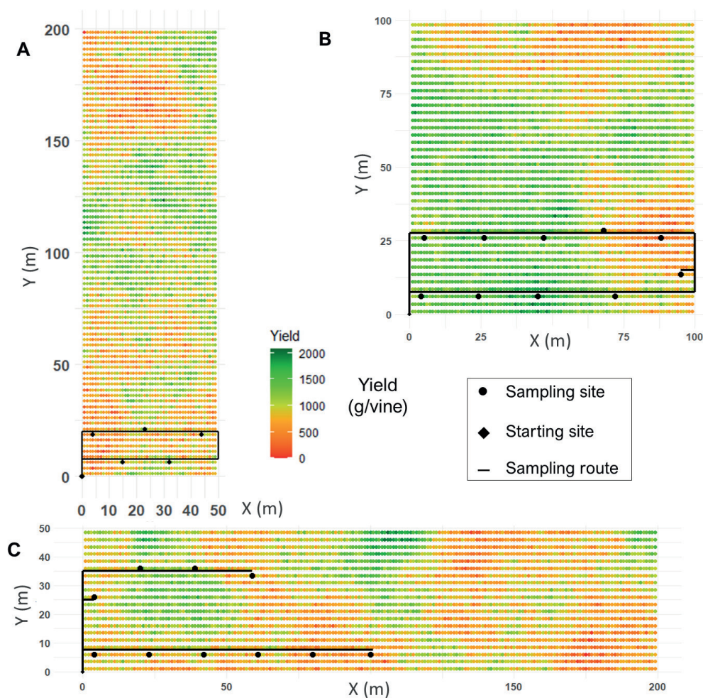
FIGURE 4. Illustration of sampling routes for three different row length
