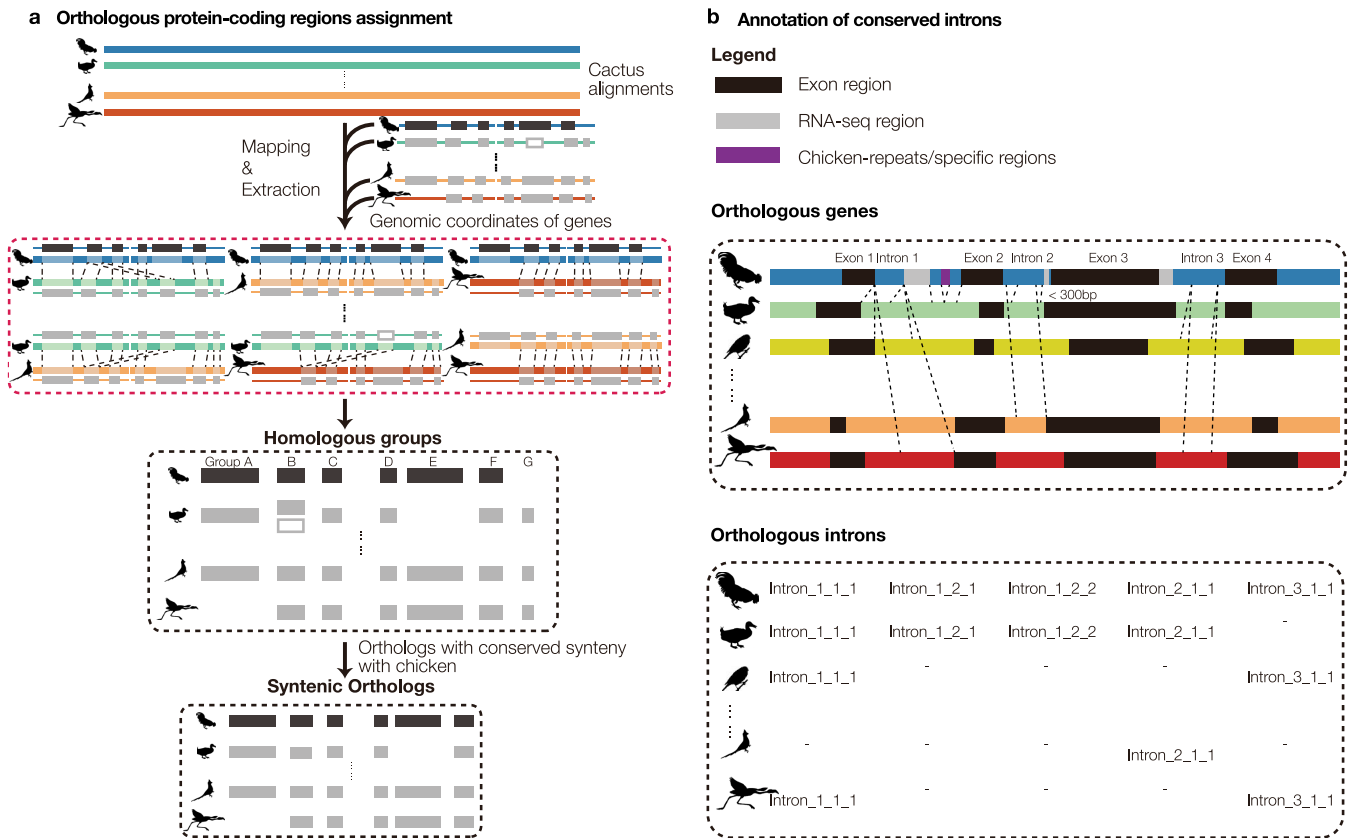
Extended Data Fig. 5 | Overview of the pipelines for identifying genomic regions. a, Assignment of orthologous protein-coding regions. All pairwise relationships between homologous regions obtained from the Cactus alignment (4 species shown here in different colours) were used to construct the homologous groups across all 363 birds. Using chicken as the reference, we further generated a table containing homologues with conserved synteny to chicken. b, Annotation of conserved orthologous intron regions on the basis of
