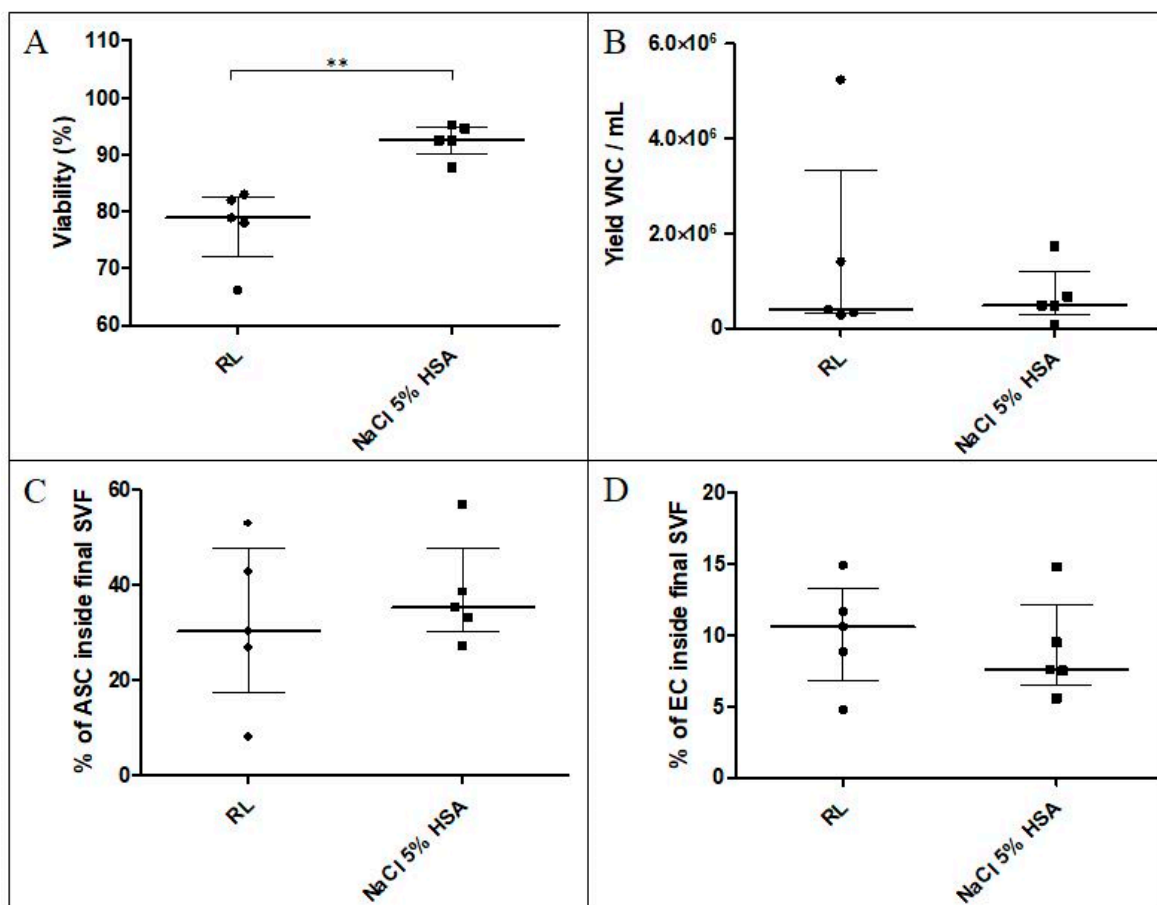
Figure 3. A ssessment of two different solutions for filtration, washing, and final resuspension of SVF. The solutions tested were RL and NaCl 5% HSA. (A) Viability was statistically higher for the NaCl 5% HSA group ( p = 0.01 ). (B) Yield of VNCs per mL AT, (C) percentage of MSCs, and (D) ECs were not statistically different. RL: Ringer's lactate; NaCl 5% HSA: saline solution enriched with HAS; VNCs: viable nucleated cells; MSCs: mesenchymal stem cells; ECs: endothelial cells. **: p = 0.01 .
