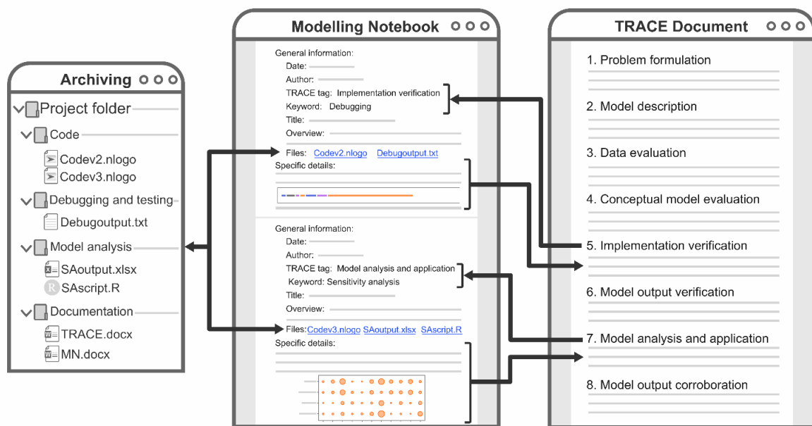
Fig. 2. Schematic figure explaining the relation between files in a modelling project, a modelling notebook, and TRACE. Notebook entries are added chronologically with tags provided by the terminology from the TRACE framework. Standardized tags and keywords, in turn, facilitate the compilation of a TRACE document from the specific details included in the notebook entries. Entries provide hyperlinks to all files related to a modelling task, indicating their location in the archiving system; TRACE terminology should also be used to organize and name files and folders.
