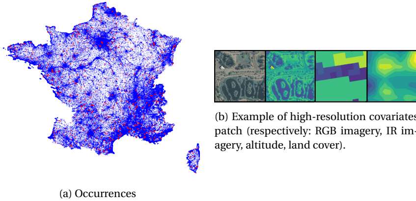
Fig. 1: Occurrences distribution (training data in blue, test data in red) in France (a), and an example high-resolution tensor (b). RGB patch is displayed with native colors, IR imagery, altitude and land cover are in artificial colors from purple (lowest values) to yellow (highest values).
