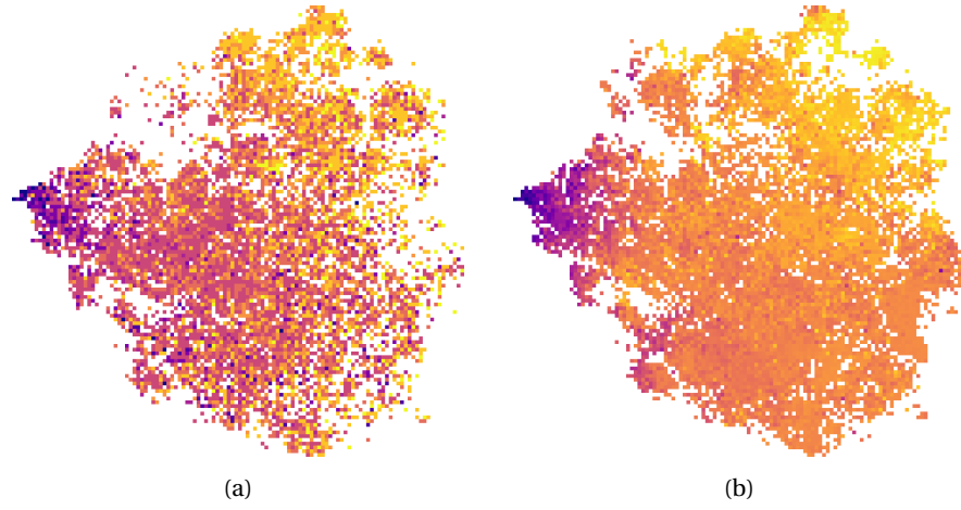
Fig. 2: Visualization of the occurrences' species preferences in temperature (EIV T)(a) and the annual mean temperature (bio_1) at occurrences location (b) on the t-SNE space. Artificial colors from purple (lowest values) to yellow (highest values).
